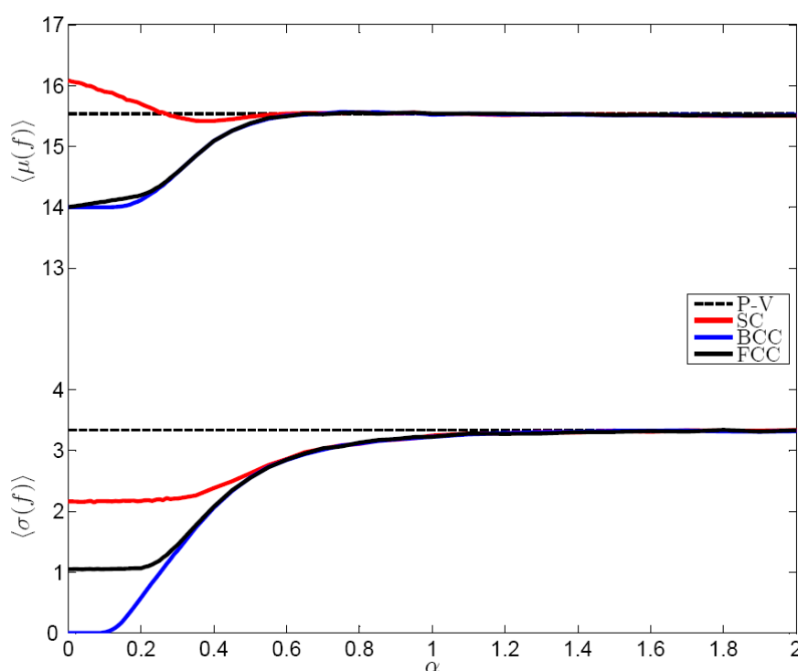
Figure 7. Ensemble mean of the mean and of the standard deviation of the number of faces of the Voronoi cells for perturbed SC, BCC and FCC cubic crystals. The error bars, whose half-width is twice the standard deviation computed over the ensemble, are too small to be plotted. The Poisson-Voronoi limit is indicated.
