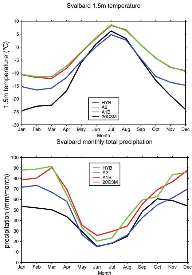
Fig. 9. Svalbard's monthly mean (area averaged) cycle of surface air temperature ( ^{\circ}\text{C} ), (a), and total precipitation ( \text{mm/month} ), (b).
