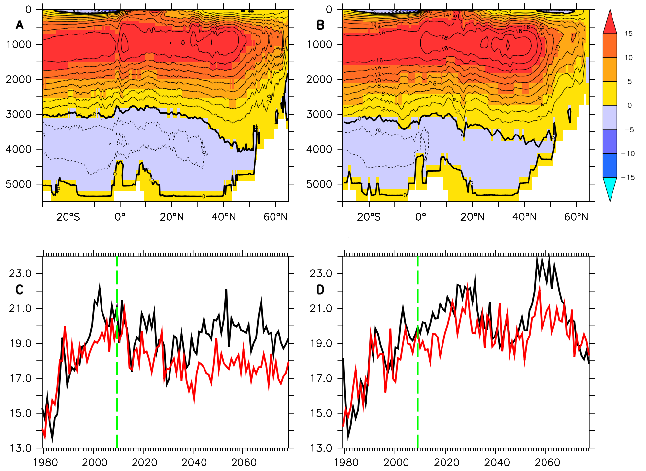
Fig. 1 Annual mean Atlantic meridional stream function (2009:2078, meridional velocity integrated from the ocean floor to a given depth) for A) HiGEM1.2 B) HadGEM1.2. C) Black line: MOC at 40°N (meridional ocean velocity integrated across Atlantic basin and from ocean floor to 1000m depth) in HiGEM1.2. Red line: Max Annual mean Atlantic meridional overturning streamfunction (i.e. panel A) at 26.7°N in HiGEM1.2. Mean depth of max is 923m for all years. D) as C, but for HadGEM1.2. Mean depth of max is 949m for all years. All units are Sv ( 10^6 m^3/s ). Green dotted line denotes 2009. All subsequent analysis is performed on data from 2009 to 2078 (unless otherwise stated) in order to exclude the initial rapid 30 year re-adjustment.
