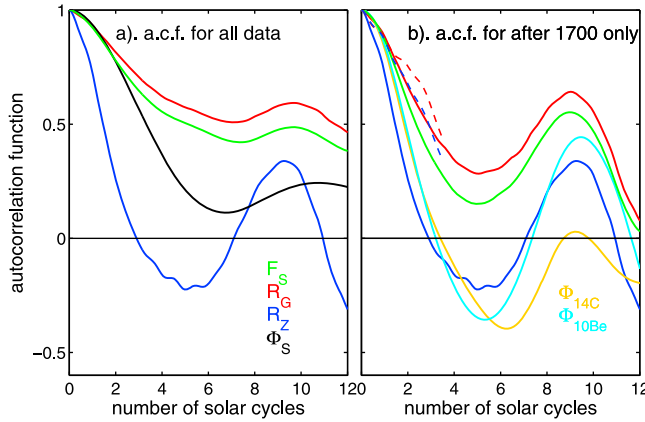
Figure 2. Auto correlation functions (ACFs) of solar activity indicators. The correlation coefficient is shown as a function of lag (in units of a mean solar cycle length of 11.1 years). (a) from 25-year running means of the group sunspot number R_G (red); the Zurich sunspot number R_Z (blue); the modelled signed open solar flux F_S (green) and the heliospheric modulation potential, \Phi_S (black) for data series that, respectively, start in 1610, 1700, 1610 and 7300BC. (b) ACFs for 10-year running means of data after 1700: red, blue and green are for R_G , R_Z and F_S and cyan and orange are for the heliospheric modulation potential from ^{10}\text{Be} and ^{14}\text{C} isotope abundances, \Phi_{^{10}\text{Be}} and \Phi_{^{14}\text{C}} , respectively. The dashed red and blue lines in Figure 2b are for R_G and R_Z (respectively) for after 1885 only.
