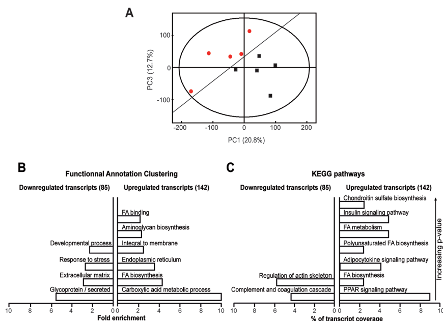
Figure 1. Transcriptomic effects of MEHP on human adipocytes. Human preadipocytes ( n = 5 ) were differentiated in vitro into adipocytes for 11 days and then treated with MEHP (100 \mu M) or DMSO (0.1%, vehicle) for 24 h. (A) PCA analysis was conducted using expression data from the entire microarray (32 322 probesets). Black: DMSO, red: MEHP. (B, C) Gene ontology analyses were conducted on the 142 significantly upregulated and on the 85 downregulated transcripts, using DAVID (B) and KEGG (C) databases. P < 0.05 was used as cutoff for selecting significantly enriched biological pathways.
