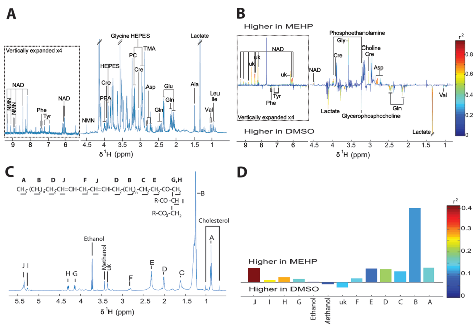
Figure 2. ^1\text{H} NMR-based metabolomic investigation MEHP effects on human adipocytes. (A) Representative ^1\text{H} NMR spectra (600 MHz) derived from an aqueous extract of human adipocytes. (B) Plot of O-PLS-DA coefficients related to the discrimination between ^1\text{H} NMR spectra from aqueous extracts of human adipocytes treated with MEHP ( n = 5 , top) vs. DMSO ( n = 5 , bottom) for 48 h. O-PLS-DA parameters: R^2X = 0.65 , R^2Y = 0.94 , Q^2Y = 0.73 , p = 9 \times 10^{-3} , one predictive and one orthogonal component. (C) Representative ^1\text{H} NMR spectra (600 MHz) derived from an organic extract of human adipocytes. uk: unknown compound. (D) Plot of O-PLS-DA coefficients related to the discrimination between ^1\text{H} NMR spectra from organic extracts of human adipocytes treated with MEHP ( n = 5 , top) vs. DMSO ( n = 5 , bottom) for 48 h. O-PLS-DA parameters: R^2X = 0.93 , R^2Y = 0.98 , Q^2Y = 0.68 , p = 0.03 , one predictive and two orthogonal components. Leu: leucine; Ile: isoleucine; Val: valine; Glu: glutamate; Gln: glutamine; Asp: aspartate; TMA: trimethylamine; Cre: creatine; PC: phosphocholine; uk: unknown compound; PEA: phosphoethanolamine; NMN: N -methylnicotinamide; NAD: nicotinamide adenine dinucleotide; Tyr: tyrosine; Phe: phenylalanine.
