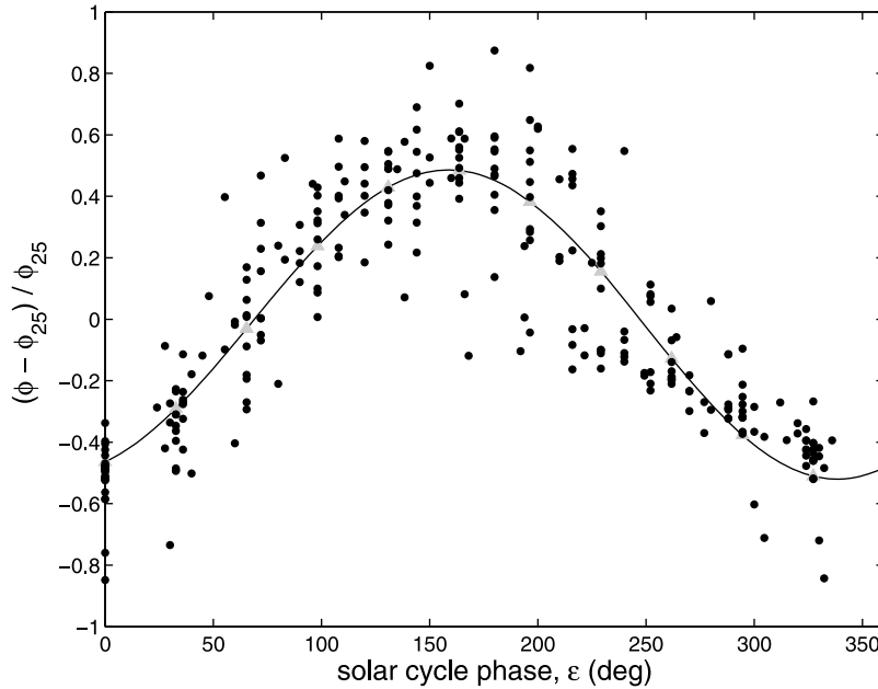
Figure 2. The variation of detrended annual means of the modulation potential \phi with solar cycle phase \epsilon . The values of the fractional deviation from 25-year means (\phi - \phi_{25})/\phi_{25} are plotted where \phi are the annual values for 1720–2000 reconstructed by Usoskin et al. [2002] and \phi_{25} is the simultaneous value derived from the 25-year means of Steinhilber et al. [2008], as also shown in Figure 1. The solar cycle phase is derived from solar minimum dates in \phi using the procedure adopted by Lockwood and Owens [2009]. Black dots are annual values and the line is the best-fit 8th order polynomial. The grey triangles give annual fitted values, assuming the solar cycle length is 11 years.
