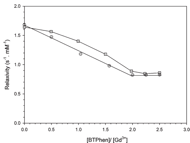
Figure 4. Nuclear magnetic relaxation dispersion (NMRD) titration curve of an anhydrous \text{CD}_3\text{CN} solution of \text{Gd}(\text{ClO}_4)_3 (○) and \text{Gd}(\text{NO}_3)_3 (□) by BTPhen 9 .
