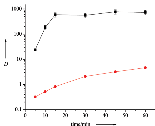
Figure 9. Extraction of Am(III) and Eu(III) from 1 M HNO 3 by BTPhen 9 in octanol (0.01 M) as a function of time (■ = D_{\text{Am}} , ● = D_{\text{Eu}} ; temperature: 22 ± 1 °C).
