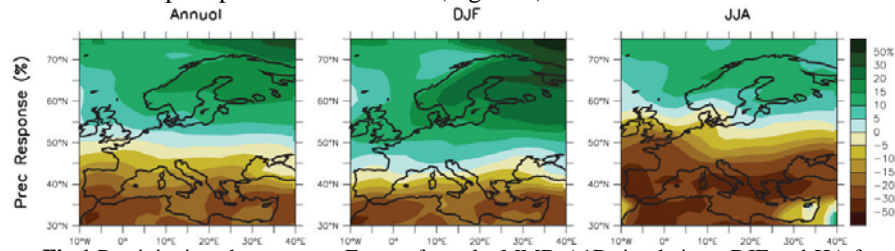
Fig 1 Precipitation changes over Europe from the MMD-A1B simulations, DJF and JJA fractional change in precipitation between 1980 to 1999 and 2080 to 2099, averaged over 21 models. Source: Christensen et al.(2007).
