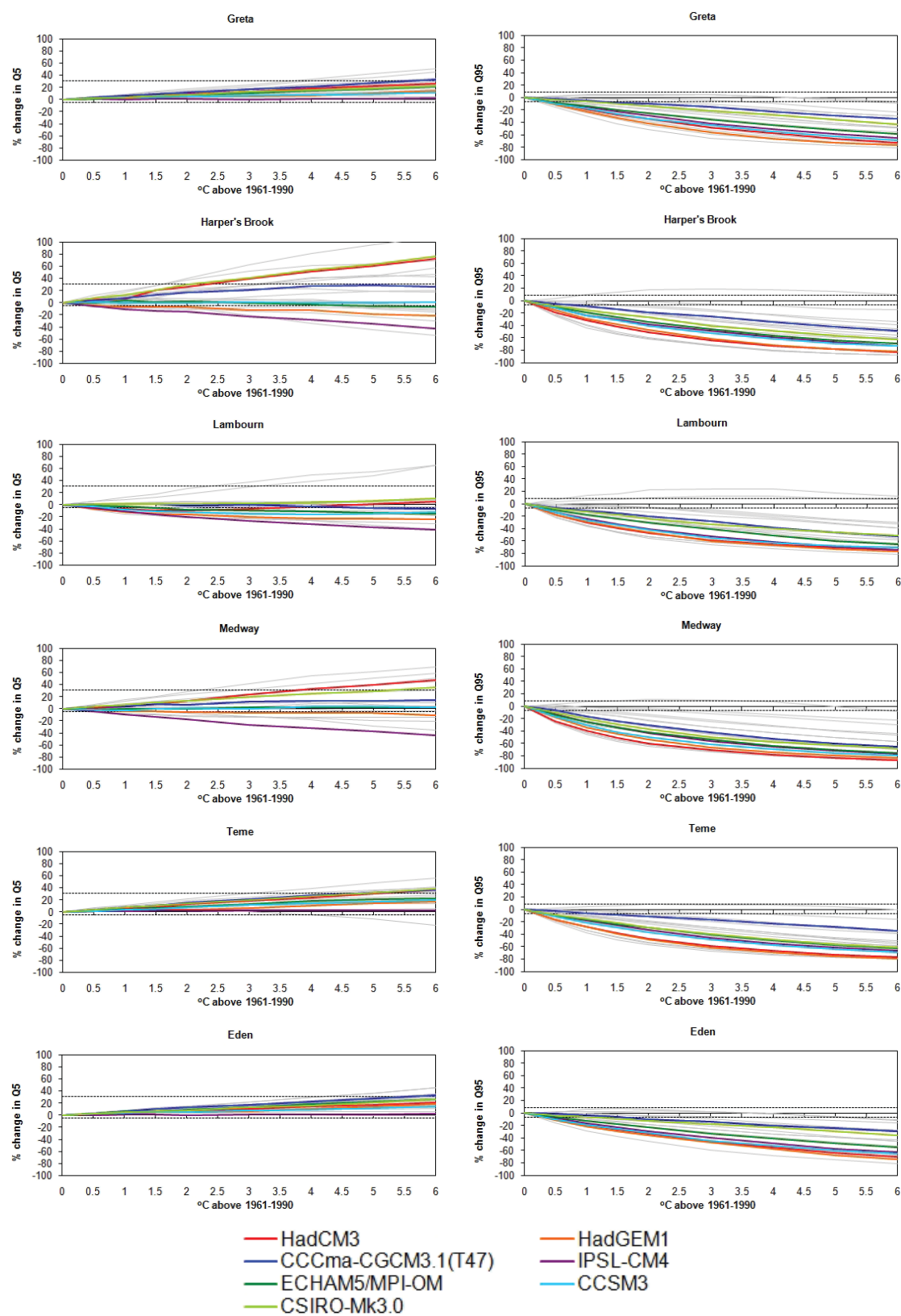
Fig. 6. Change in Q95 and Q5 in each catchment. The seven priority climate model patterns are highlighted.
