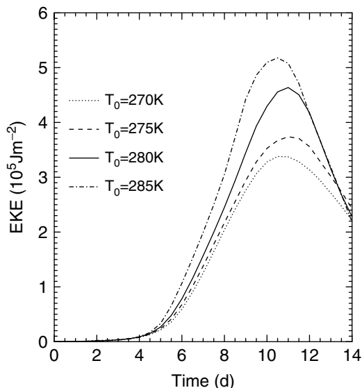
Figure 8. Time series of eddy kinetic energy for various values of the initial surface temperature at 45^\circ\text{N} (shown on the plot).
