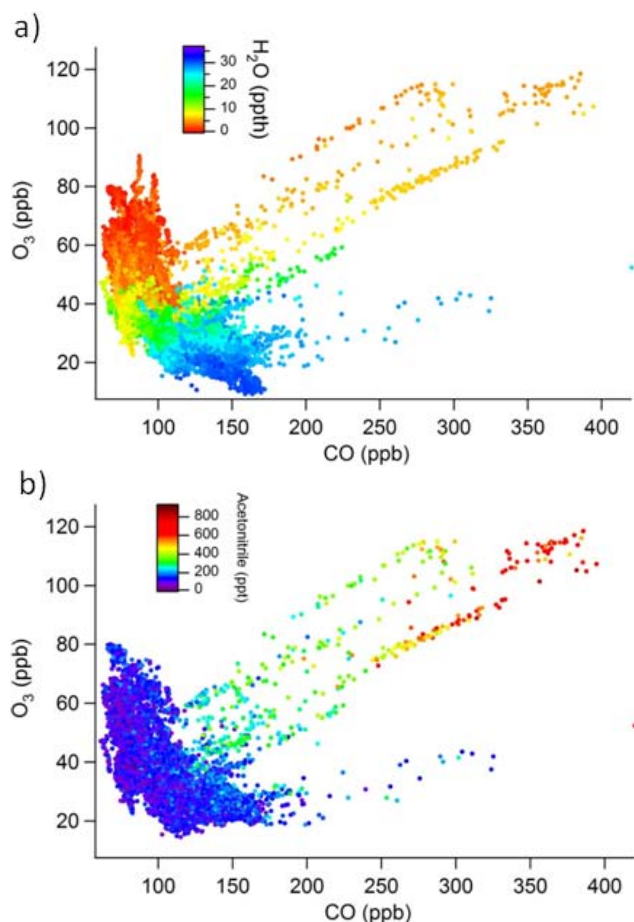
Fig. 7. Ozone and CO correlations coloured by a) water vapour and b) acetonitrile. Data from the BAe-146 only.
