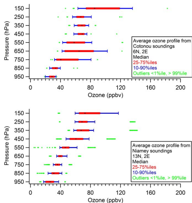
Fig. 11. Average ozone profiles based on (top) 9 soundings from Cotonou ( 6^{\circ} N, 2^{\circ} E) launched at 10:00 or 11:00 a.m. local time between 21 July and 22 August 2006 and (bottom) 29 soundings from Niamey ( 13^{\circ} N 2^{\circ} E) between 26 July and 25 August 2006. The black marker is the median, the red box the range of the 25 to 75 percentiles, the blue whiskers the range of the 10 to 90 percentiles and the green markers are less than the 1 percentile and greater than the 99 percentile.
