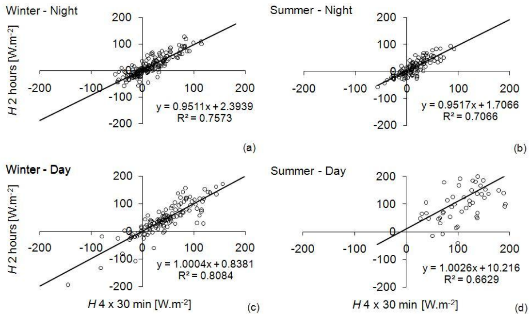
Figure S4: Sensible heat fluxes calculated using block-averaging of 2-h and 30 min (mean of the four periods). (a) Winter night, (b) summer (night), (c) winter day and (d) summer day.
