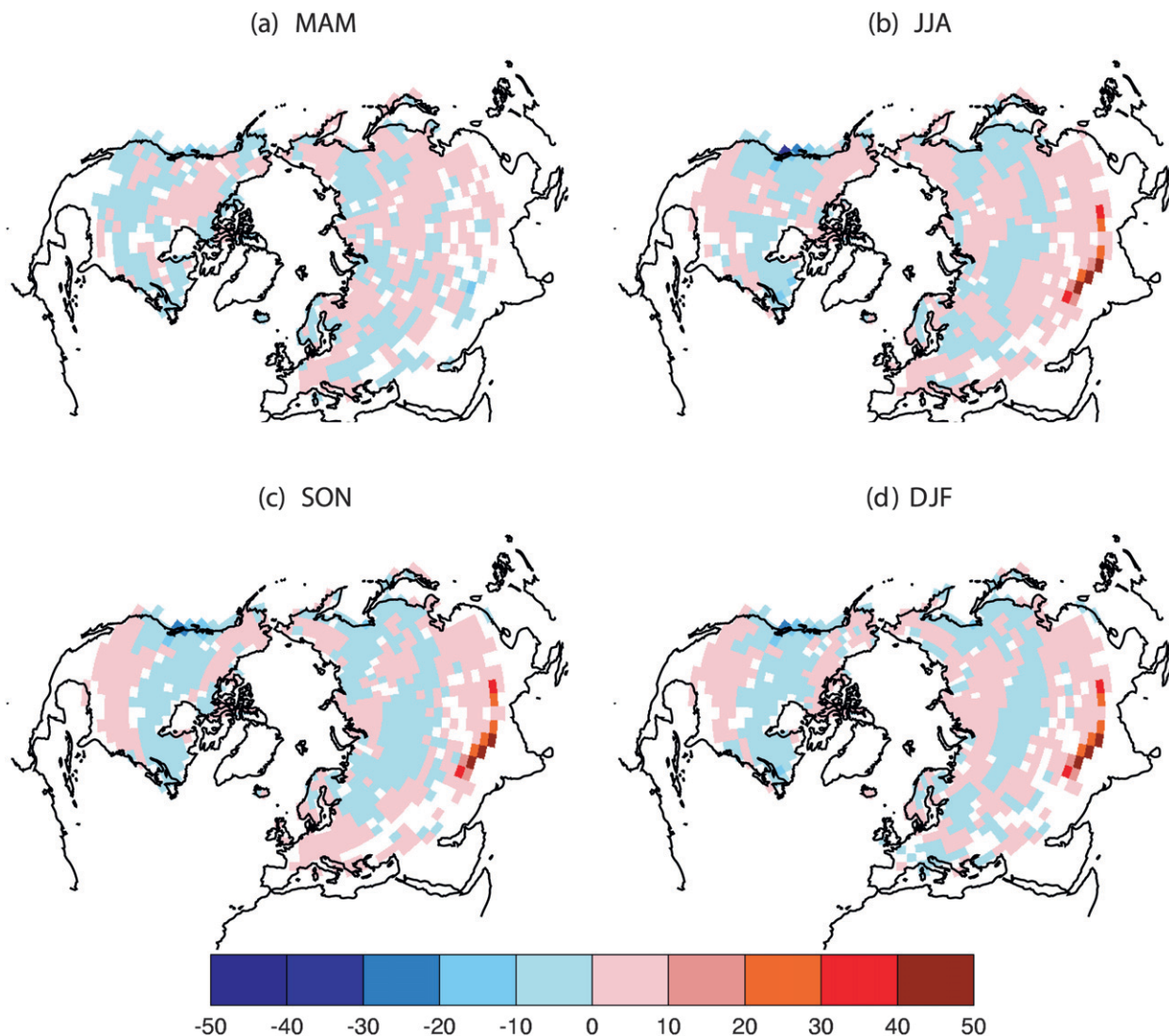
FIG. 3. February SWE anomaly distribution (mm) from years with positive ENSO index in the previous (a) MAM, (b) JJA, (c) SON, and (d) coincident DJF.
