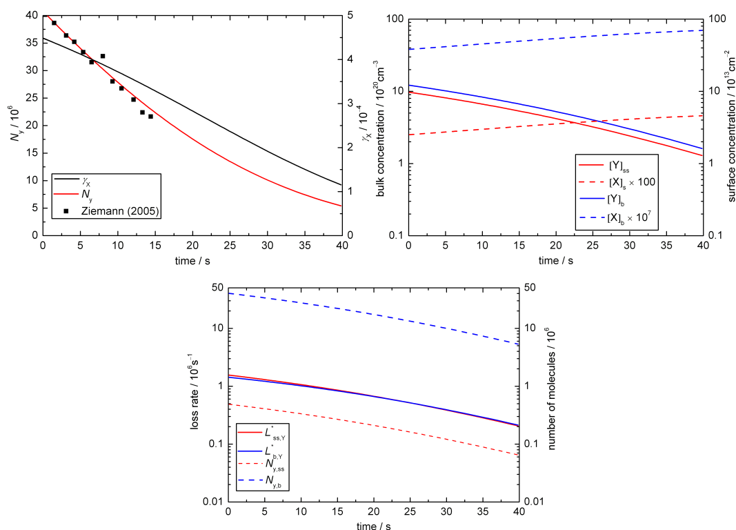
Fig. 8. Temporal evolution of aerosol particle composition and kinetic parameters in base case 2 (BC2; X = O 3 , Y = oleic acid): (a) ozone uptake coefficient ( \gamma_x ) and total number of oleic acid molecules ( N_y ; symbols indicate experimental data from Ziemann, 2005); (b) surface and bulk concentrations (square brackets); (c) numbers of oleic acid molecules at the surface and in the bulk of the particle ( N_{y,ss} , N_{y,b} ) and corresponding absolute loss rates ( L_{ss,Y}^* = L_{ss,Y} \times A_{ss} , L_{b,Y}^* = L_{b,Y} \times V_b ).
