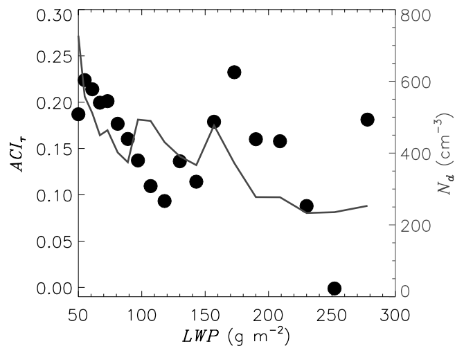
Figure 4. Relationship of (symbols, left ordinate) ACI and (line, right ordinate) N_d to increasing LWP. ACI_{\tau} is calculated for 10% increasing LWP bins in the range of 50–300 g m -2 and N_d derived using equation (2). Note the general reduction in N_d with increasing LWP for values < ~150 g m -2 , and highly variable ACI_{\tau} at LWP > ~150 g m -2 . Under the latter conditions, ACI_{\tau} is more reflective of scavenging processes than aerosol effects on cloud microphysics.
