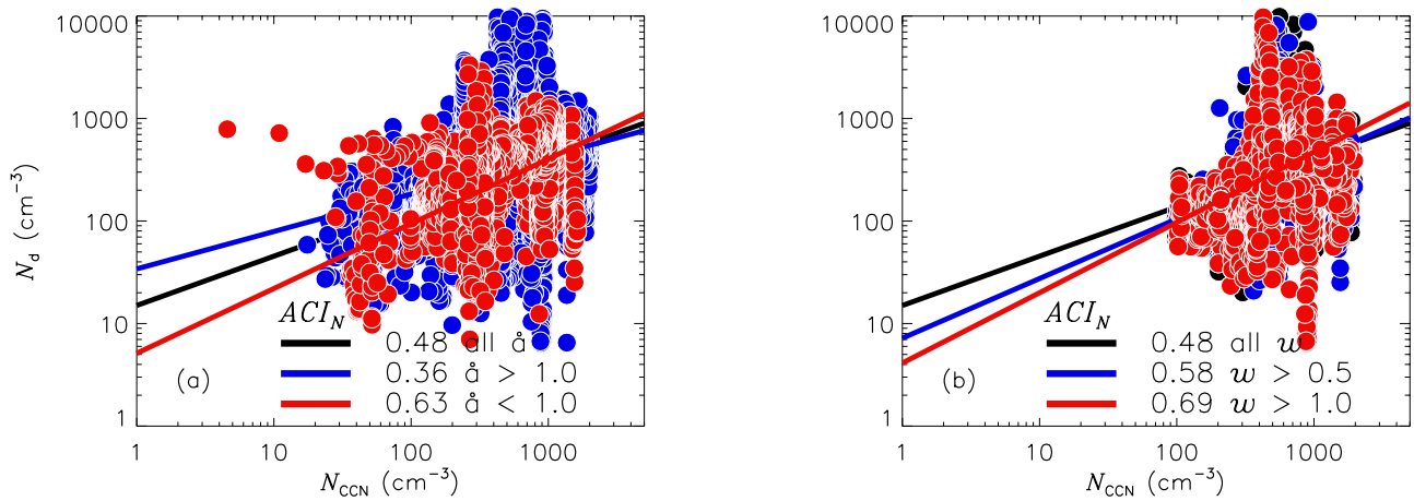
Figure 7. Differences in ACI_N for naturally varying parameters (a) Ångström exponent \hat{a} and (b) updraft velocity w (in \text{m s}^{-1} ).
