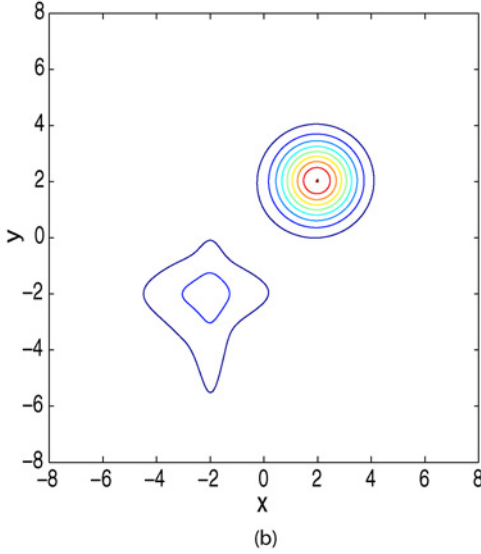
Fig. 15. (a) A GMM estimate and (b) its contour plot for the 2-D example of the Gaussian and the Laplacian mixture.
