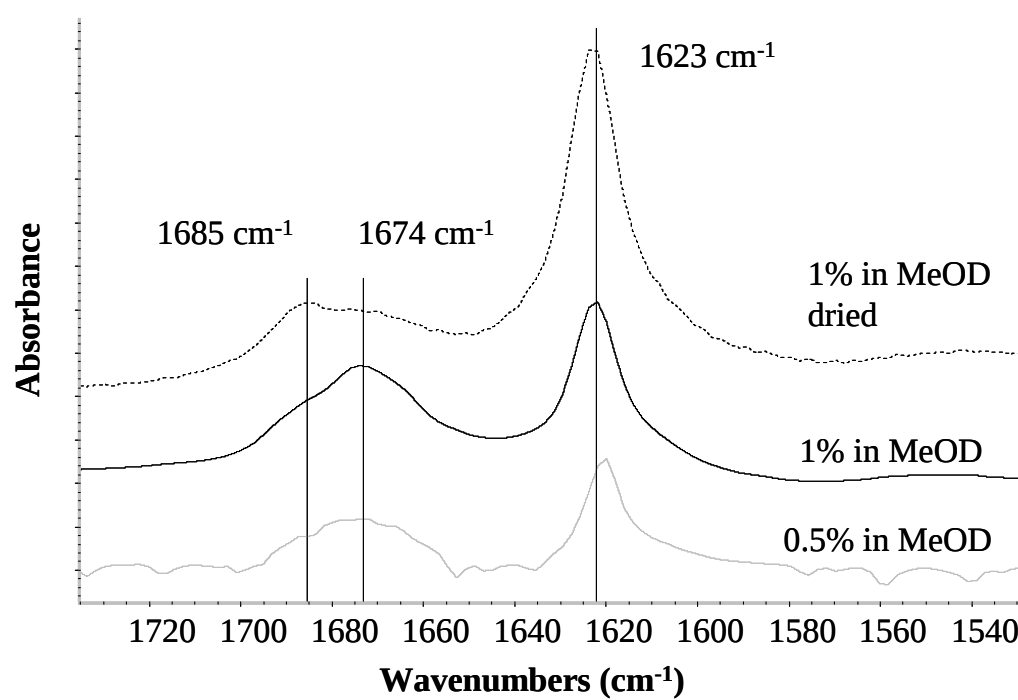
Figure 6. FTIR spectra of the amide I region of FFKLVFF in d 4 -methanol (.5% and 1% wt). The solvent spectrum has been subtracted from the spectra of the peptide solutions. The spectrum of the peptide film was also obtained
