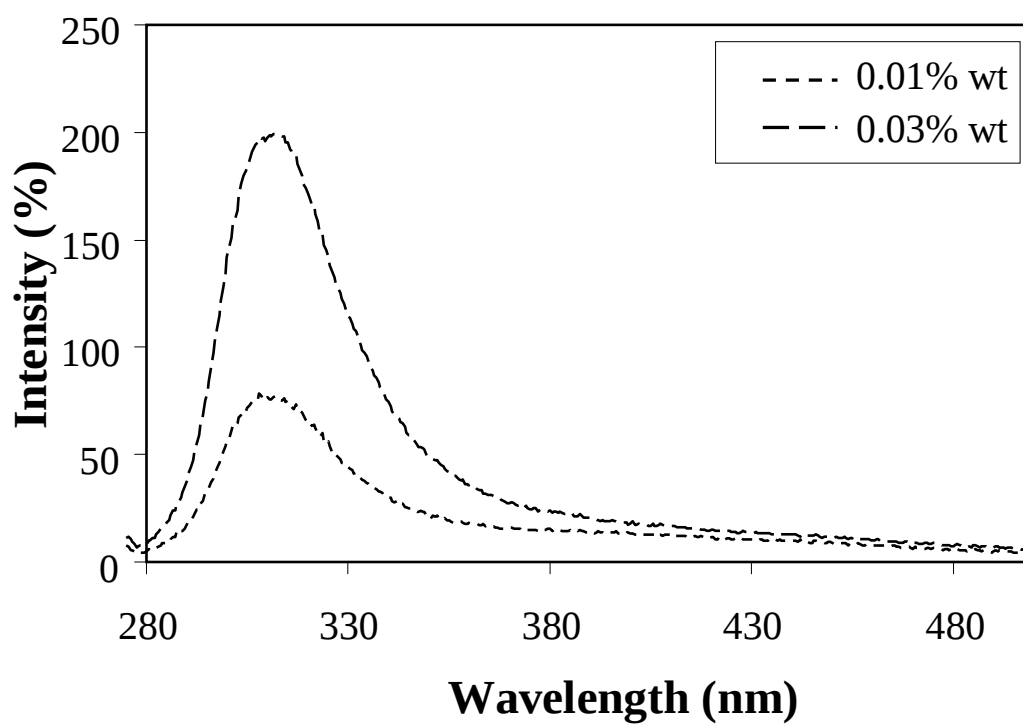
Figure 4 Fluorescence spectra showing aromatic interaction in FFKLVFF
