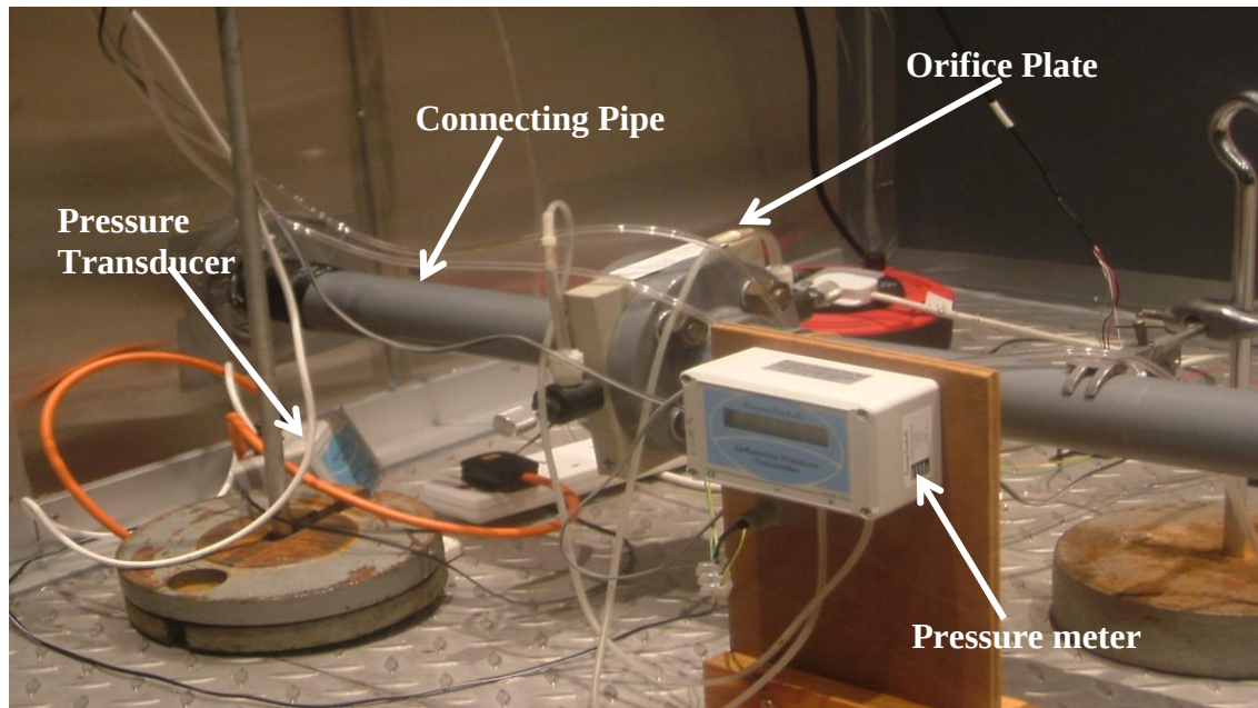
Figure 8. The set-up of the orifice plate within the environmental chamber
