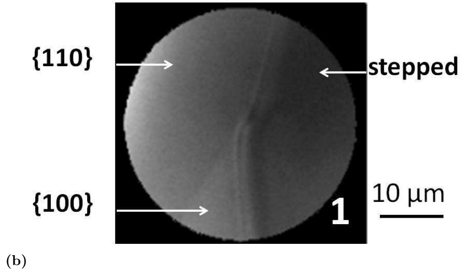
FIG. 2: (color online) (a) NEXAFS spectra from the three facets observed in region 1 after exposure to 20 L of oxygen at 373 K; (b) X-PEEM image of region 1 (photon energy 529 eV).
