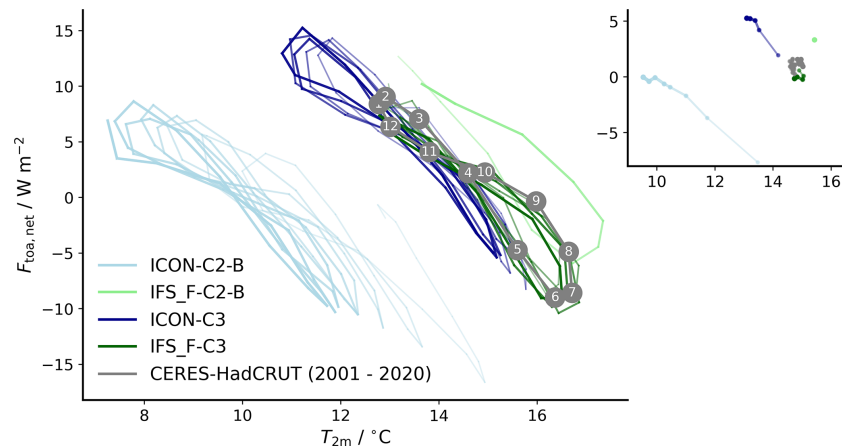
Figure 3. Annual cycles of the monthly mean 2 m temperature and top-of-atmosphere radiation balance from ICON-C2-B, ICON-C3, IFS_F-C2-B, and IFS_F-C3. Note that the radiation balance is computed as the difference of the downwelling and upwelling radiation, i.e., F_{\text{toa},\text{net}} = F_{\text{toa},\text{sw}}^{\downarrow} - F_{\text{toa},\text{sw}}^{\uparrow} - F_{\text{toa},\text{lw}}^{\uparrow} (Mauritsen et al., 2022). The widths and opacities of the lines increase with time. Gray line shows the observational reference averaged over 2001 to 2020, i.e., 2 m temperature from HadCRUT (Morice et al., 2021) and radiation balance from CERES-EBAF (Loeb et al., 2018). The months are labeled with numbers. The corresponding annual means are shown in the top-right inset. Like for the annual cycles, the widths and opacities of the lines increase with time.
