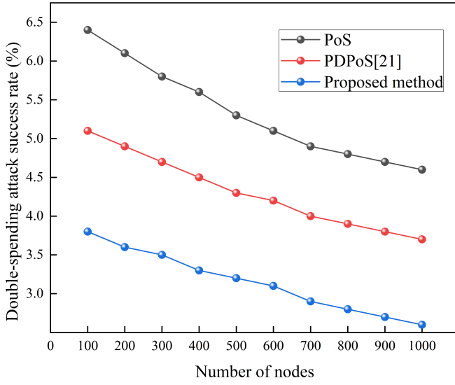
Fig. 15. Comparison of double-spending attack success rate under different numbers of nodes
