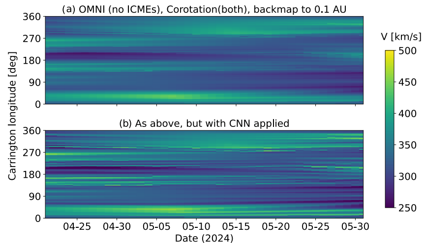
Figure 9. Example of the solar wind conditions at 0.1 AU, reconstructed around the time of the May 2024 storms. V is shown as a function of Carrington longitude and time. (a) interplanetary CMEs at AU are removed from the OMNI observations. Full longitudinal coverage at 1 AU is then obtained by corotating structures forward and backwards in time from the available OMNI observations (as shown in Figure 7e). The longitudinal profiles at 1 AU are then mapped back to 0.1 AU, accounting for the assumed acceleration profile. (b) Same as a, but the convolutional neural network is also applied to account for stream interactions between 0.1 and 1 AU.
