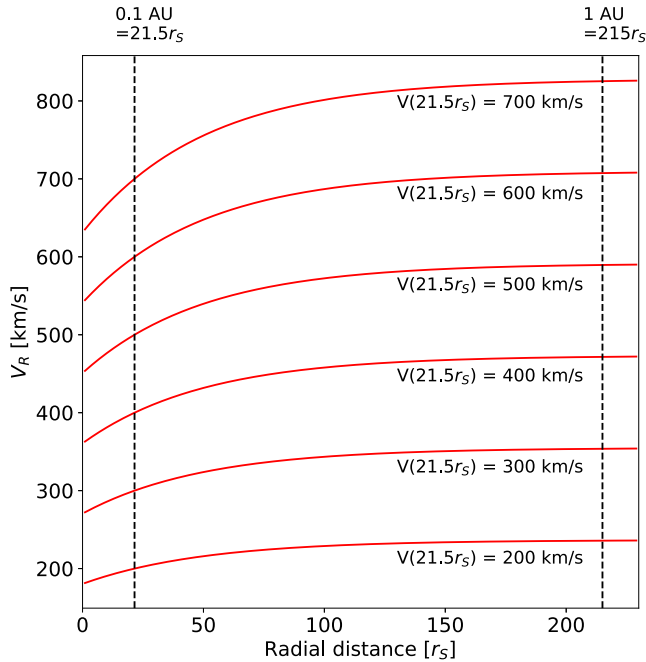
Figure 4. The solar wind acceleration profile used in the HUXt solar wind model for a range of initial speeds at the model inner boundary.
