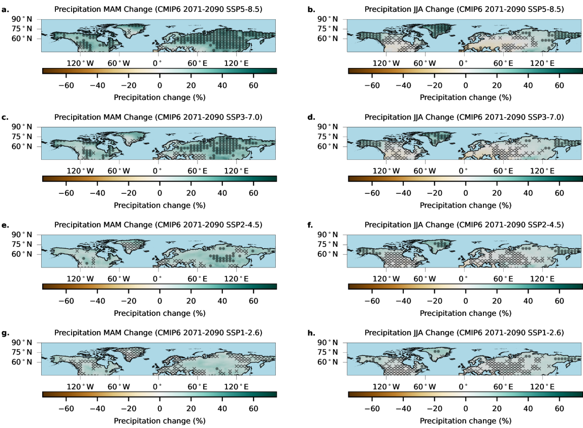
803 Figure S11: As for main paper Extended Data Figure 7A/B but for SSP5-8.5, SSP3-7.0, 804 SSP2-4.5 and SSP1-2.6
