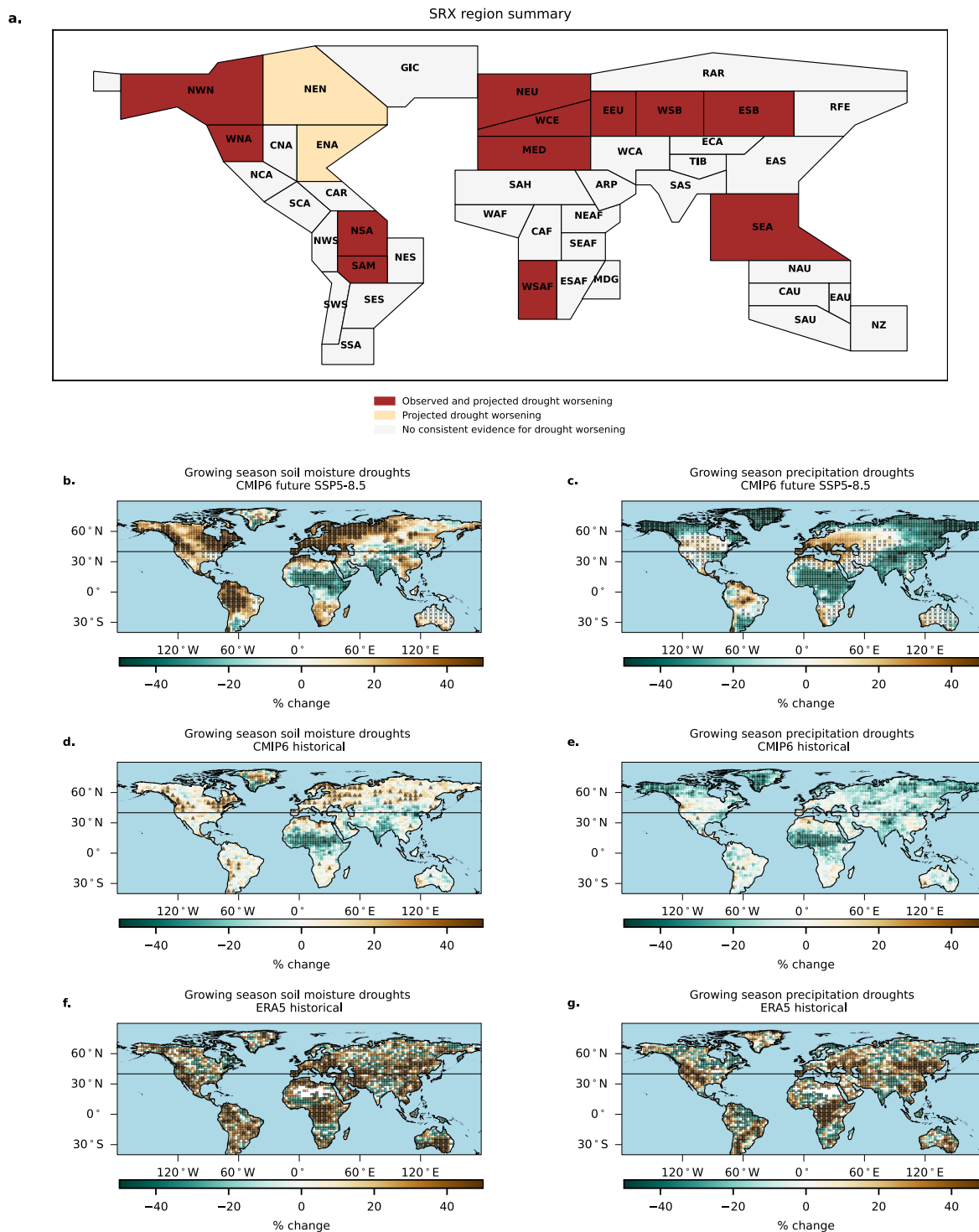
Figure 6: Emerging hotspots of agricultural drought a. SREX regional summary: each region classified as observed and projected increase in soil-moisture-defined drought, projected increase only, or no evidence of worsening (see colour key). b.–c. CMIP6 SSP5-8.5 change in growing-season drought occurrence, 2071–2090 c.f. 1981–2000, for soil moisture events (b.) and precipitation events (c.). d.–e. Historical CMIP6 change, 2001–2020 c.f. 1981–2000,
