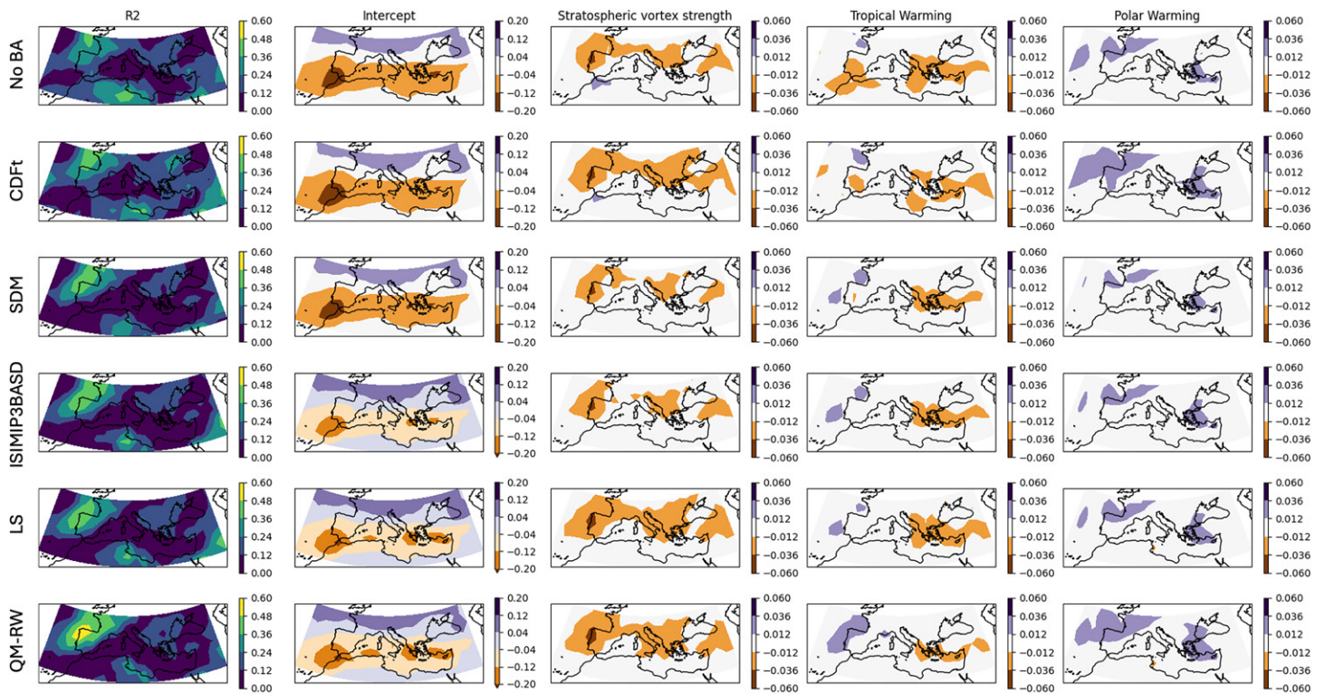
FIG. A1. Regression R2 as well as the influence of stratospheric vortex strength, tropical warming, and polar warming on the climate model ensemble spread for precipitation [ \text{mm} (\text{day K})^{-1} ] for the raw climate model ensemble and for the bias-adjusted climate models.
