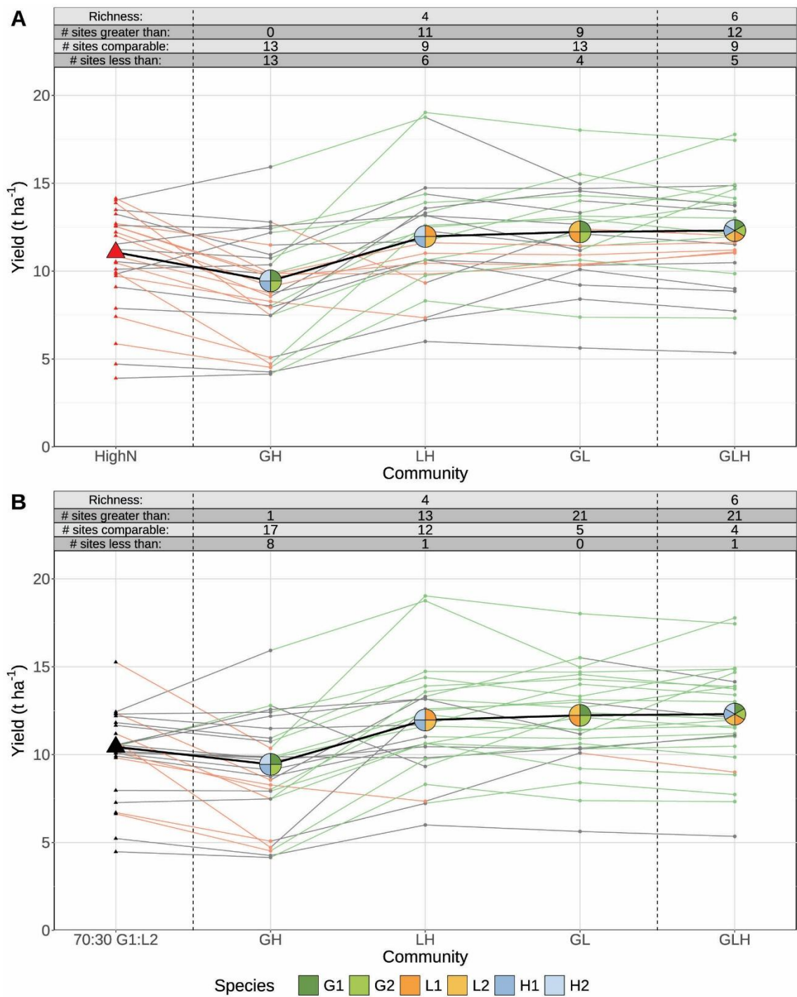
Fig. S7. Yields of four- and six-species equi-proportional mixtures were generally greater than, or comparable to, the high N grass and the 70:30 G1:L2 community at individual sites, despite high site-to-site variability. Predicted yields of selected communities across sites (black line and pie-glyphs) and at each site (colored lines and smaller points): the high N grass monoculture (red triangle), the 70:30 G1:L2 community (black triangle); the four-species equi-proportional grass-herb (GH), legume-herb (LH) and grass-legume (GL) mixtures; and the six-species equi-proportional GLH mixture (1/6:1/6: 1/6:1/6: 1/6:1/6 for G1:G2: L1:L2: H1:H2). The four species communities are arranged in
