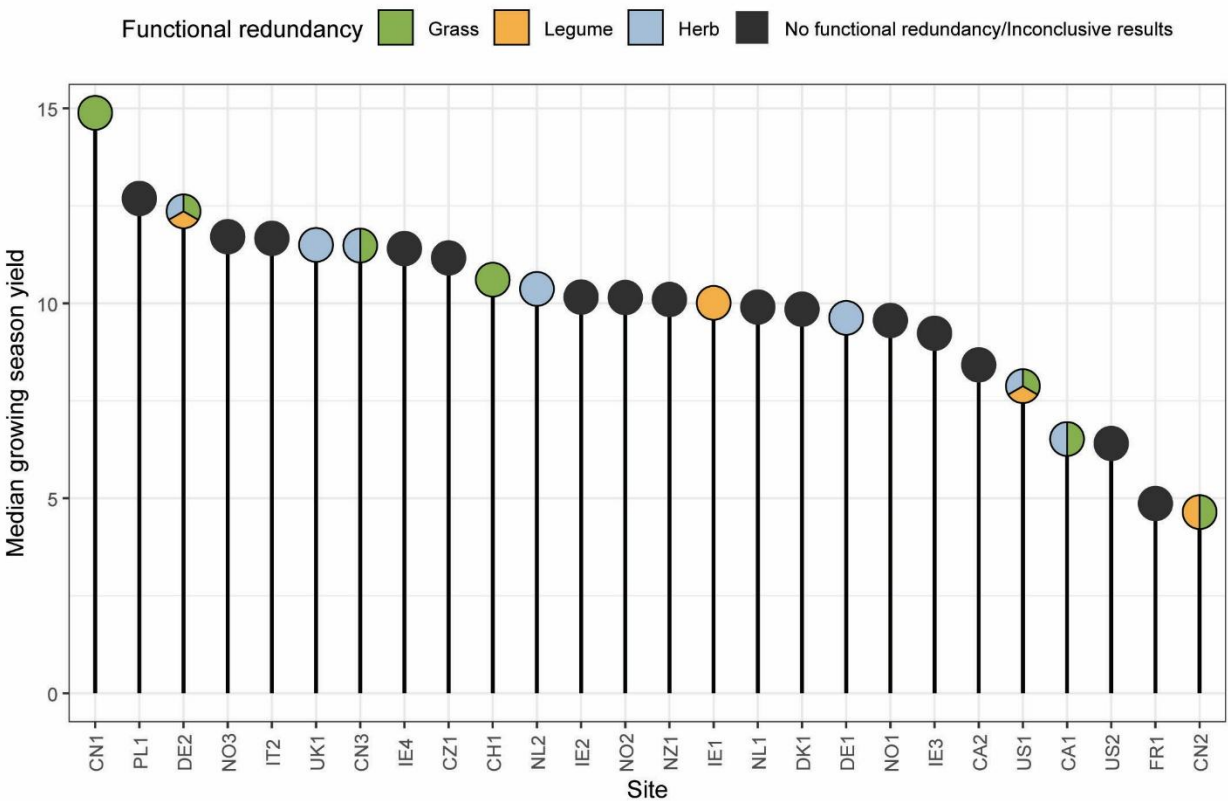
Fig. S3. Functional redundancy within functional groups. The presence/absence of functional redundancy between the two grass (green), the two legume (orange), and the two herb (blue) species at each site is shown using pie-glyphs. The pie-glyphs with green, orange and/or blue in them indicate the presence of functional redundancy between the species from the respective functional groups, while those colored in dark grey represent sites with no redundancy (or inconclusive results) between the pair of species in each functional group (details in (27)). The sites along the x-axis are arranged in decreasing order of their median yields.
