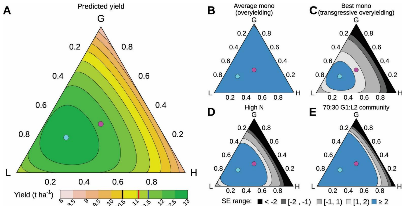
Fig. 3. Higher yields from increased plant diversity. (A) Ternary diagram illustrating predicted yield ( \text{t ha}^{-1} ) across all sites as the sown proportions of the three functional groups vary, and with the two species within each functional group sown in equal proportions to each other. Note that the vertices of the ternary are two-species communities of grasses (G), legumes (L), or herbs (H), not monocultures of individual species. The highest predicted yield is marked by a cyan circle (with sown functional group proportions: G:L:H = 24:59:17 and corresponding sown species proportions = 0.12: 0.12: 0.295: 0.295: 0.085: 0.085). In the yield legend, values are marked for the predicted responses of the 70:30 G1:L2 community (black), the high N grass monoculture (red), and the highest yielding monoculture (blue). The predicted yield for the equi-proportional six-species mixture is shown by a magenta circle. The remaining panels show the difference (measured in standard errors) of the predicted yield in A from: (B) the weighted average monoculture (for the component species at each point in the ternary; overyielding), (C) the highest yielding monoculture (i.e., L1, which was T. pratense at most sites; transgressive overyielding), (D) the high N grass monoculture, and (E) the 70:30 G1:L2 two-species community, where G1 is L. perenne and L2 is T. repens at most sites. For example, a point on panel D within the highest contour level (colored blue) represents a mixture whose predicted yield is more than two standard errors greater than the predicted yield of the high N grass monoculture. The six-species equi-proportional mixture and the optimal mixture are marked in B to E for comparison to panel A.
