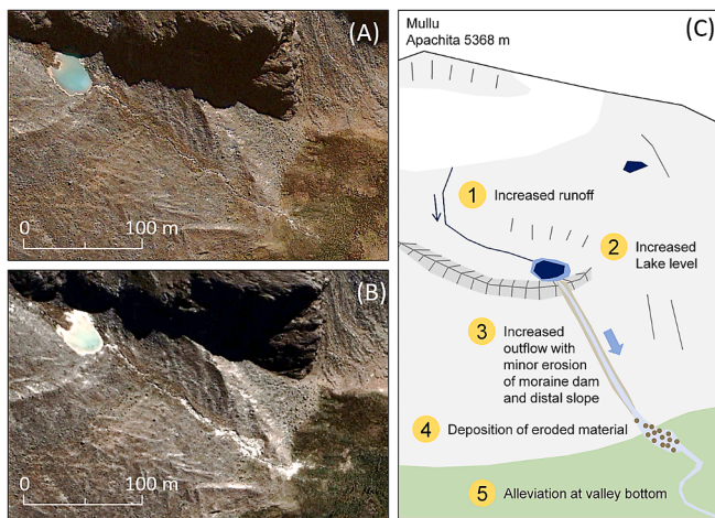
Fig. 10. An example of a low magnitude GLOF in the C. Real, Bolivia (for location see Fig. 4). (A) shows the lake before the GLOF (Google Earth Maxar Technologies image from 20th June 2010) while (B) shows the post-event situation with visible erosional and depositional areas located downstream the lake (Google Earth Maxar Technologies image from 18th May 2016). (C) summarises the process chain associated with this event.
