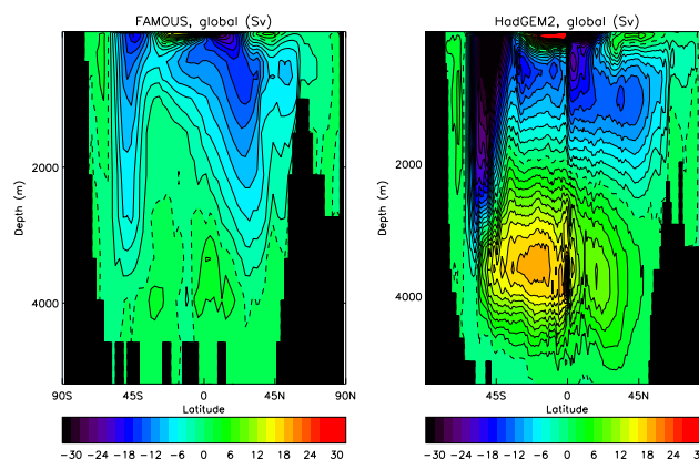
Figure 9. Global meridional overturning circulation (MOC) in FAMOUS (left) and HadGEM2-ES (right). The zero contour is dashed.
