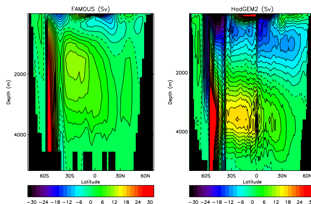
Figure 11. Pacific meridional overturning circulation (MOC) in FAMOUS (left) and HadGEM2-ES (right). The zero contour is dashed.
