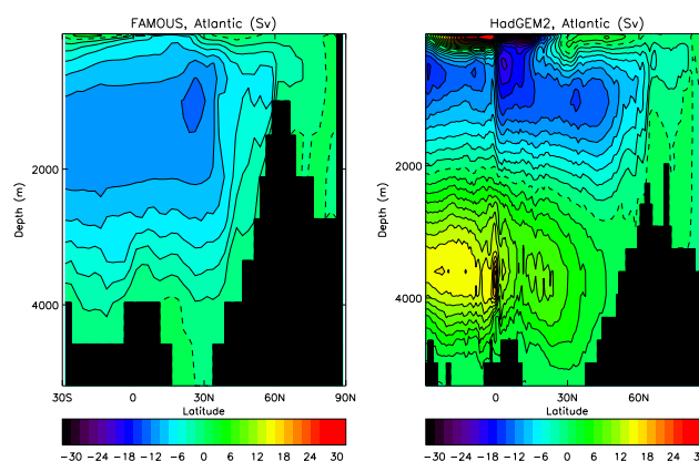
Figure 10. Atlantic meridional overturning circulation (MOC) in FAMOUS (left) and HadGEM2-ES (right). The zero contour is dashed.
