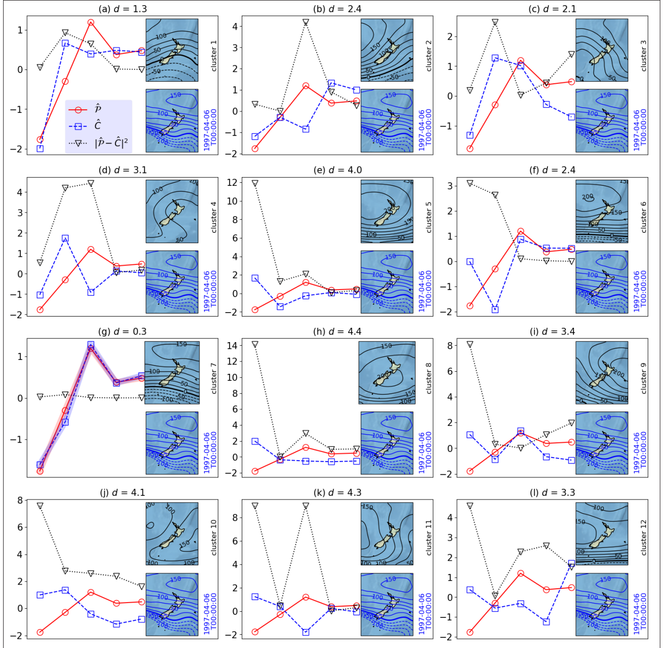
Figure A.1: Geometrical illustration of how an arbitrary observation of z (here at 0000 UTC on the 6th of April 1997) can be fitted to pre-existing clusters. Each subfigure shows the same arbitrary observation of geopotential height in the blue contours and the black contours show the 12 separate clusters obtained from this analysis (Figure 3 and Figures 5 (a) and (b)). As shown in the text, we want to find the smallest Euclidean distance, d , between the projection of the observation onto the EOFs, \hat{P} (○), and the cluster means, \hat{C} (□) as given by Equation 6. Note the simplified nomenclature used - i.e. lack of subscripts - to improve clarity. The individual |\hat{P} - \hat{C}|^2 values are also shown (▽). The square root of the sum of the |\hat{P} - \hat{C}|^2 values gives the Euclidean distance, d , shown in the subfigure titles and (g) highlights the similarity of the blue and red lines and hence the lowest d value.
