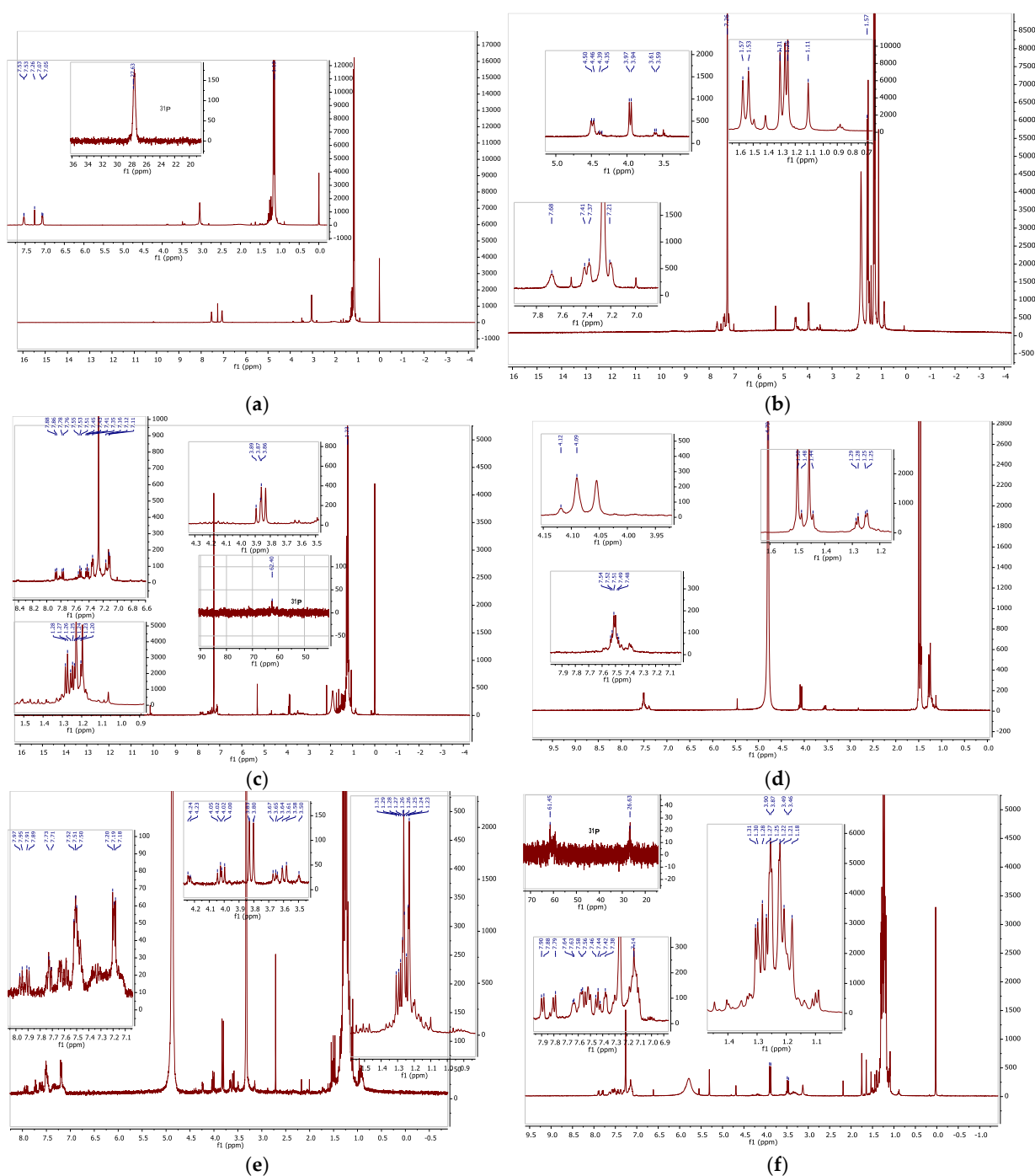
Figure 10. (a) ^1\text{H} NMR of compound 1 with ^{31}\text{P} NMR inset (b) ^1\text{H} NMR of compound 4 in \text{CDCl}_3 . (c) ^1\text{H} NMR of compound 4 in wet ( \text{D}_2\text{O} ) \text{CDCl}_3 , with resonance expansions. (d) Compound 4 in \text{D}_2\text{O} . (e) Compound 4 in methanol- \text{d}_4 . (f) ^1\text{H} NMR of compound 4 in \text{CDCl}_3 with added pyridine- \text{d}_5 , with ^{31}\text{P} NMR inset. For additional information please see the Supplementary Materials section.
