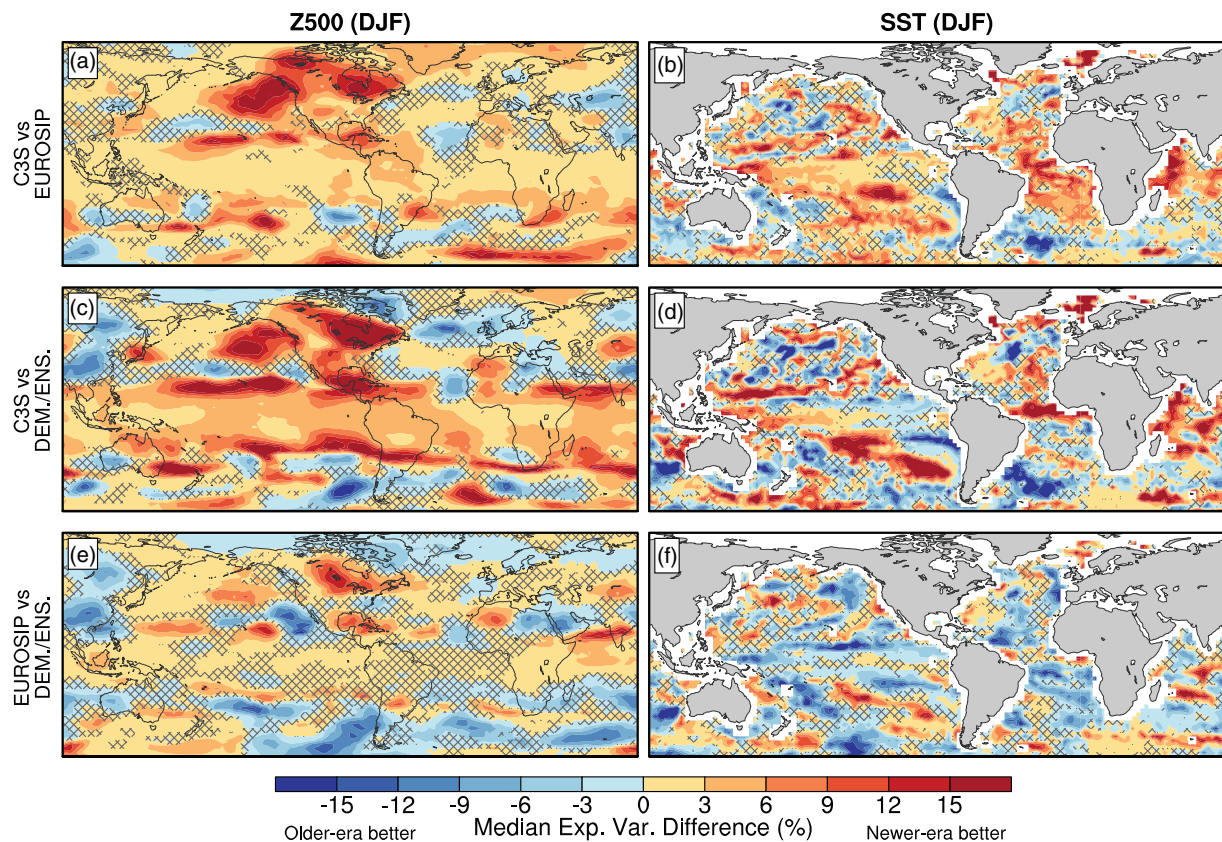
FIGURE 7 Maps of model-era skill comparison for Z500 and SST for boreal winter hindcasts (DJF). At each grid point, the colour shows the median difference in explained variance of the ensemble mean hindcast correlation skill (i.e., \Delta r^2 ) over the distribution of model era comparisons (similar to the approach in Figures 5 and 6). These were calculated, as before, after controlling for the same forecast period and ensemble size. The hatching indicates grid points where the Bayes factor is less than 100, when comparing between model eras. As before, the Bayes factors were calculated for the median of the distributions by repeated subsampling (see Section 2). [Colour figure can be viewed at wileyonlinelibrary.com ]
