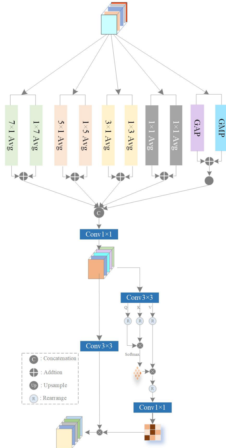
Figure 2. The structure of the Multi-scale Pooling Feature Perception (MPFP).
