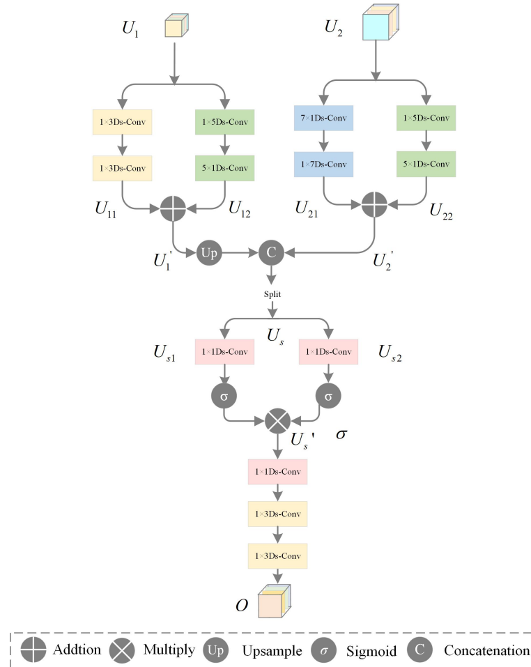
Figure 6. The structure of the Multi-scale Feature Convolution Fusion (MFCF).
