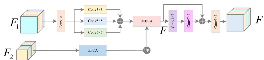
Figure 3. The structure of the Bilateral Feature Mixed Attention (BFMA).
