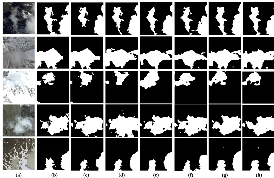
Figure 12. Comparison of segmentation results on the HRC_WHU dataset. (a) Test image; (b) Ground truth; (c) MFMANet; (d) OCRNet; (e) ACFNet; (f) PSPNet; (g) DeepLabV3+; (h) DFN. In this figure, black represents background, and white represents cloud.
