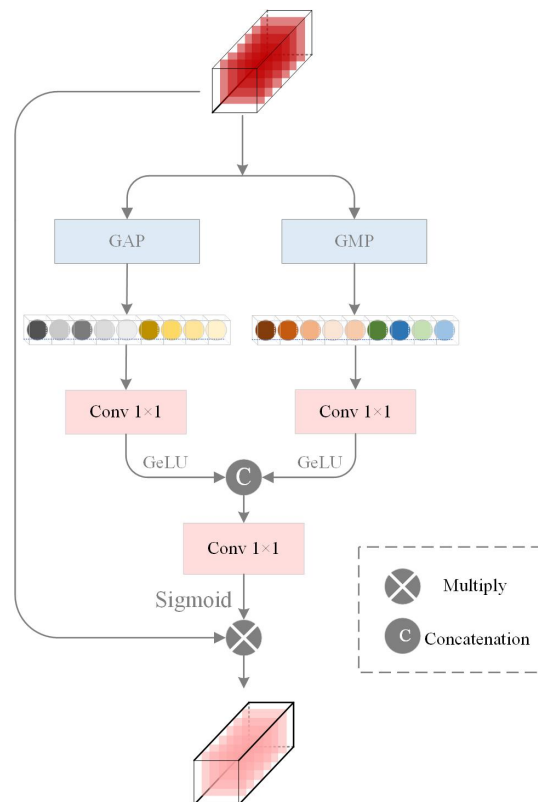
Figure 4. The structure of the Global Feature Channel Attention (GFCA) module.
