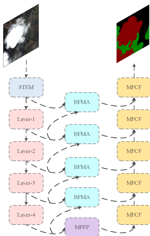
Figure 1. The overall structure of the Multi-scale Feature Mixed Attention Network (MFMANet).
