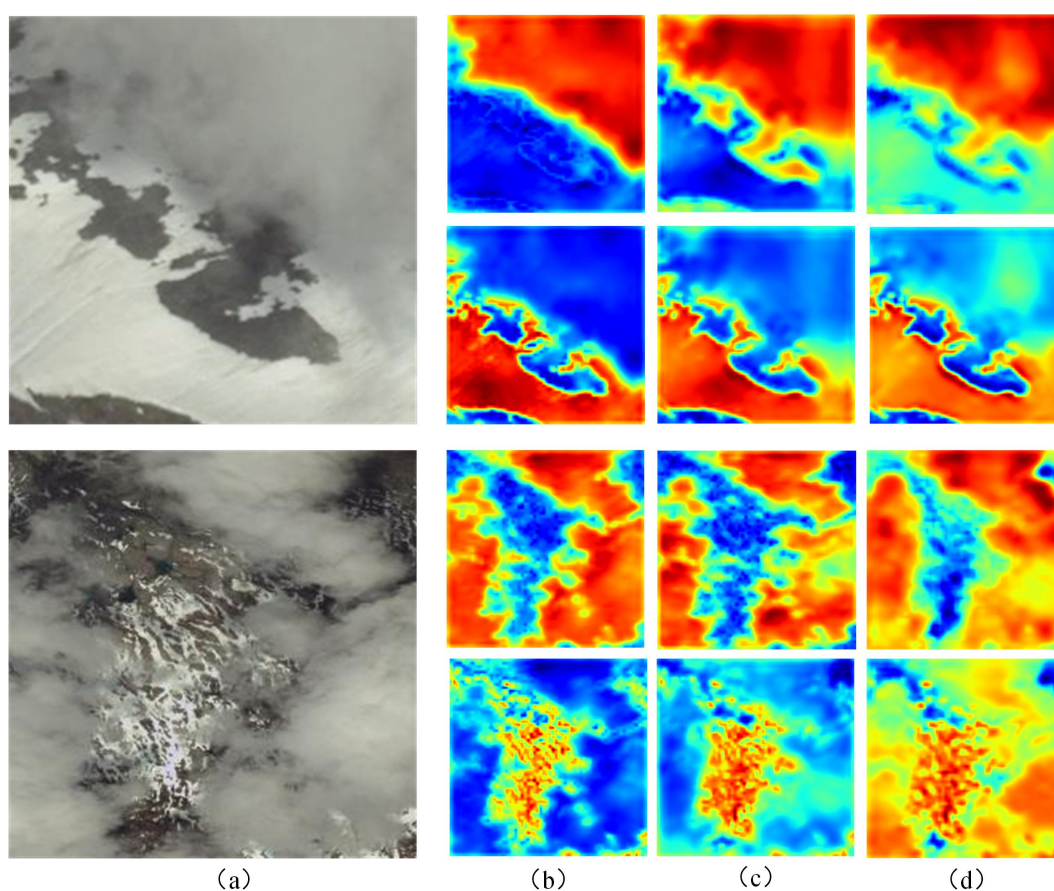
Figure 9. Heatmaps of cloud and snow under different module combinations. (a) Test image; (b) MPFP + BFMA + MFCF; (c) MPFP + BFMA; (d) MPFP.
