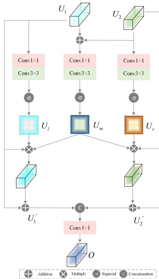
Figure 5. The structure of the Multi-Branch Spatial Aggregation (MBSA) module.
