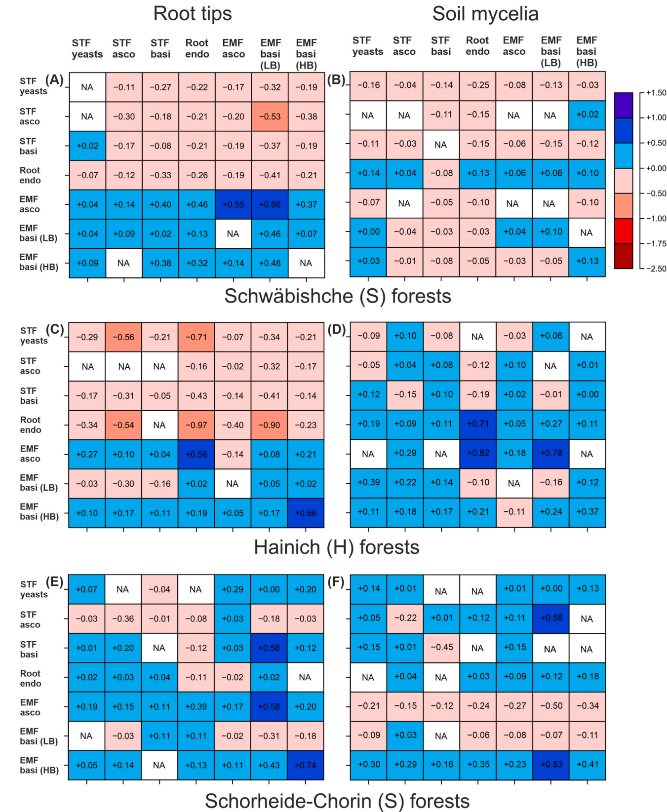
Fig. 4. Global interaction influence ( \beta_{ij} ) of guild j on guild i calculated across all samples in the three regions: S = Schwäbische Alb (A, B), H = Hainich-Dün (C, D), and S = Schorheide-Chorin (E, F). In the root (the left columns) and soil mycelium (the right columns) fungal communities. The interacting guilds j is represented by x-axis (columns) and i by y-axis (rows) names. The grey NA cells represent uncertain interactions. EMF = ectomycorrhizal fungi, STF = saprotrophic fungi, HB = high-biomass mycelium fungi, LB = low-biomass mycelium fungi. Number of plot replicates: n = 30 in A, 25 in H, and 29 in S.
