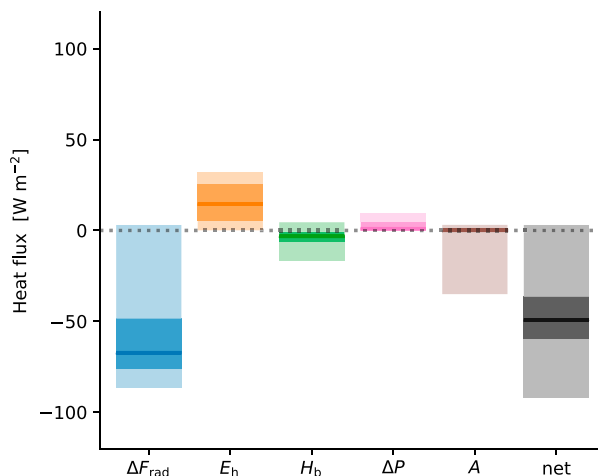
FIG. 6. Full-drift bulk mixed-layer heat budget as calculated over all 58 MOSAiC RCML cases. The abscissa labels refer to the terms as defined in section 2c, with the last column being the net tendency. For each term, the median is indicated by the thick horizontal line, and the interquartile and 5th–95th percentile ranges are indicated by medium and light shading, respectively. The term \Delta F_{\text{rad}} is the difference in the net LW radiative flux measured across the liquid cloud layer. The term E_h is the downward sensible heat flux at z_h , and H_b is the upward sensible heat flux at z_b . The term \Delta P is the difference in precipitation flux across the bulk layer. The term A is the vertically integrated tendency of horizontal heat advection. The term “net” is the net total tendency of all terms combined.
