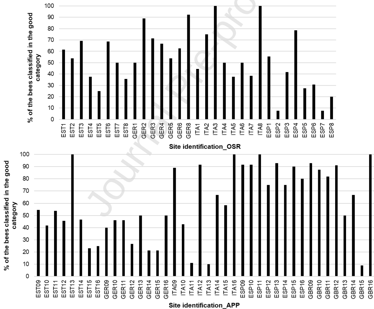
Fig. 3. Percentage of bees classified in the correct category at each site for OSR (top) and APP (bottom). Estonia (EST), Italy (ITA), Germany (GER), Spain (ESP) and Great Britain (GBR)
