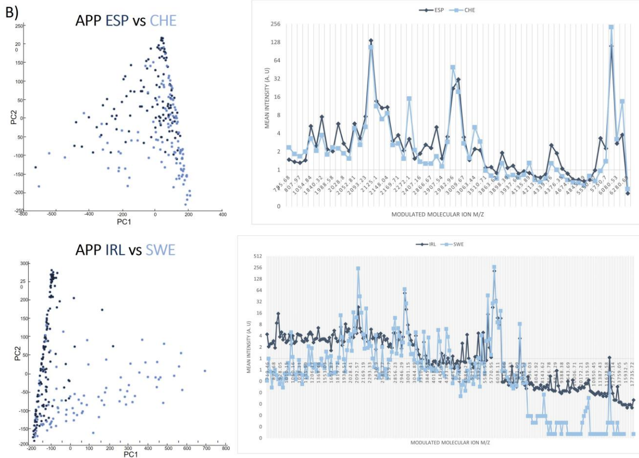
Fig. 2. Principal component analysis of individuals (left graphs) with the lowest and highest modulated molecular ions (MMIs, right graphs) and their corresponding distribution (Log2-transformed) in OSR (A) and APP (B). ITA Italy, IRL Ireland, GBR Great Britain, EST Estonia, ESP Spain, CHE Switzerland, and SWE Sweden. Each point represents one haemolymph MFP from an individual bee.
