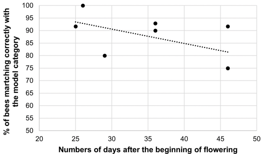
Fig. 5. Percentage of correct recognition of the site condition depending on the date after the start of flowering, in the case of Spain with Apple crop. Each point represents the average percentage of recognition for each site.
