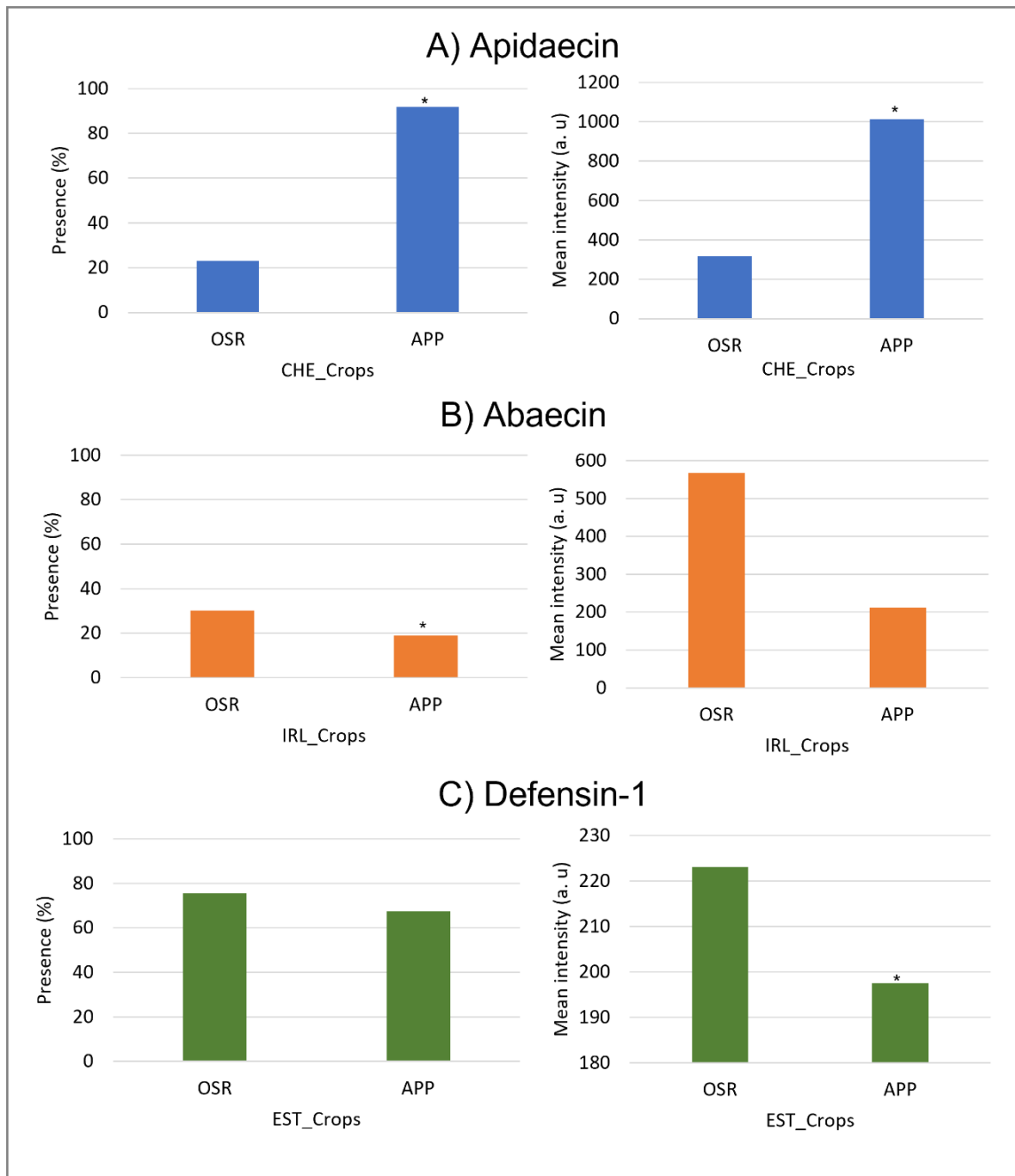
Fig. 7. Variations of the antimicrobial peptides in CHE Switzerland, IRL Ireland and EST Estonia in the studied crops oilseed rape (OSR) and apple (APP). A) Apidaecin, B) Abaecin and C) Defensin-1. * p-value < 0.05.
