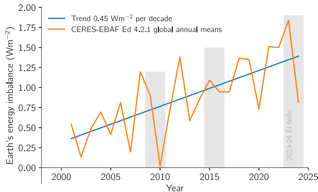
Figure 1. Annual global mean energy imbalance observed from space during 2001–2024. The imbalance is derived from the CERES-EBAF Edition 4.2.1 data set (Loeb et al., 2018). The blue line shows the linear trend over the 2001–2024 period when full annual means are available. Gray shading shows years affected by major El Niño events.
