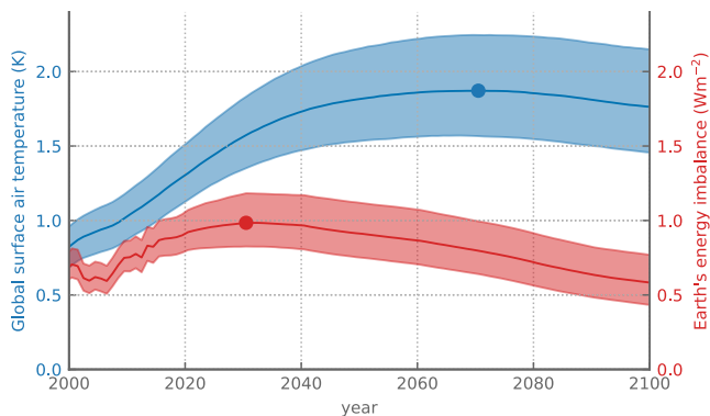
Figure 2. Climate model global mean temperature and energy imbalance under a strong mitigation scenario meeting the 2° target (SSP1-2.6). Time series are estimated from the IPCC AR6 Earth system emulator (IPCC, 2021, Chapter 7 supplementary material). Displayed data are from (Meyssignac et al., 2023). Uncertainty ranges indicate the 90 percent confidence interval of the spread caused by uncertainties in forcing, the climate response, and the carbon cycle. The displayed uncertainty range therefore excludes internal variability. The dots mark the peak year on each time series.
