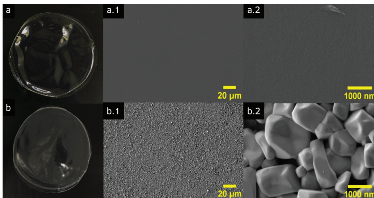
Figure 1. Appearance of PVA-based film manufactured using the casting method. (a) pristine PVA film; (a.1) PVAC-500x; (a.2) PVAC-20,000x; (b) PVA NISIN 5,000 \text{IU mL}^{-1} ; (b.1) PVA NISIN-500x; (b.2) PVA NISIN-20,000x.
