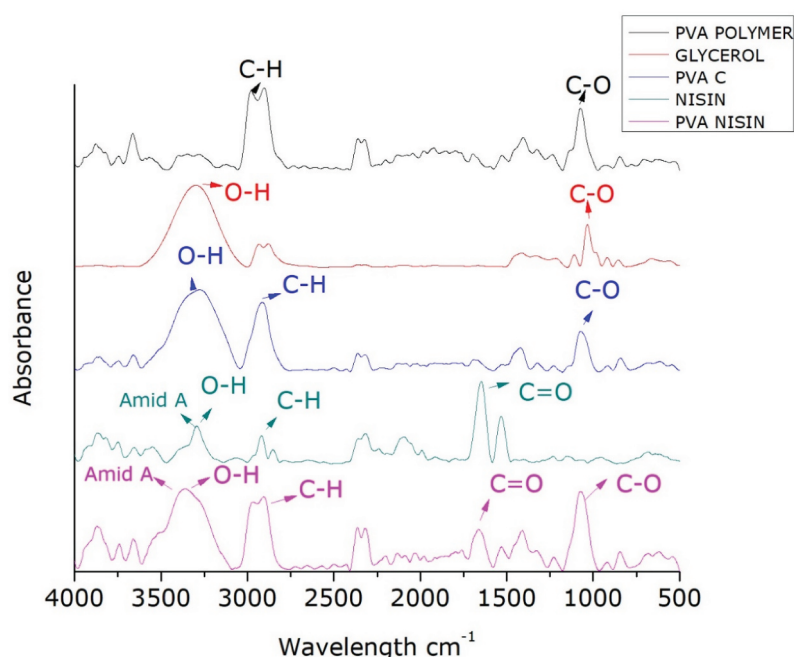
Figure 3. FT-IR spectroscopy of individual and aggregate compounds in polymeric matrices.
