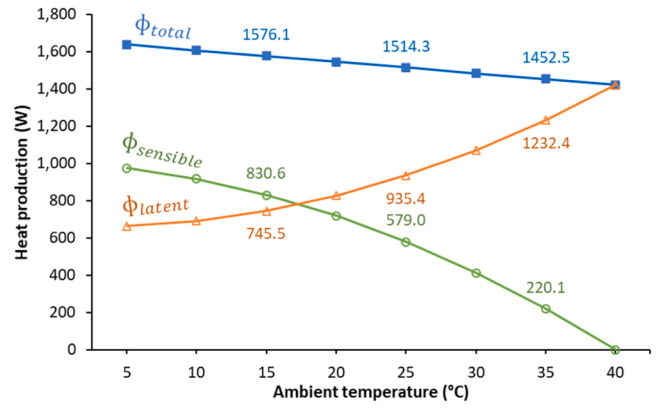
Fig. 3. Changes in a dairy cow's total heat production, sensible and latent heat dissipation with increasing ambient temperature ( T ).
