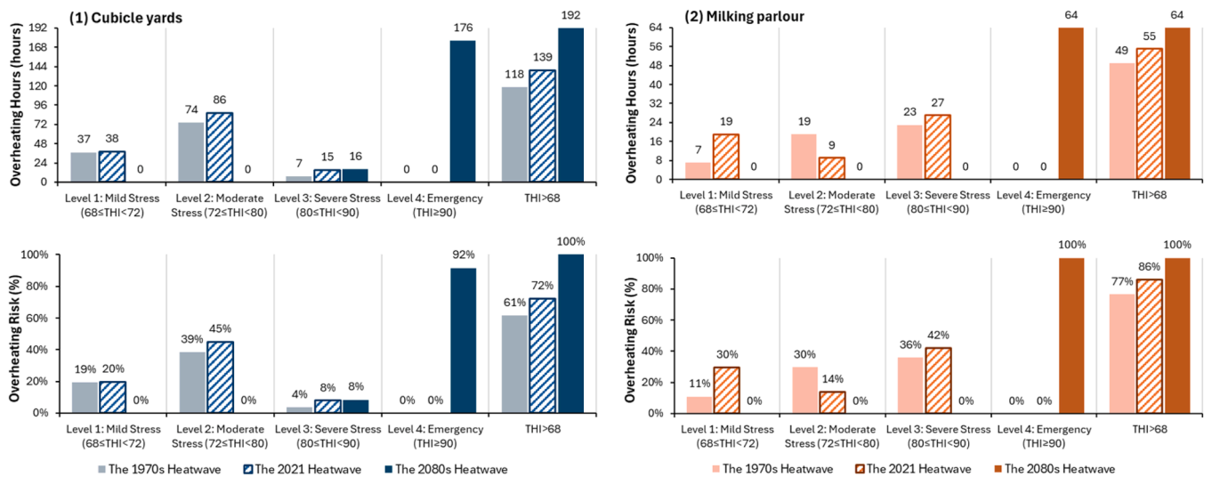
Fig. 11. Heat Stress Hours and Heat Stress Risk (%) in response to changing heatwaves for the cubicle yards (occupied throughout the day) and milking parlour (occupied during the milking times: 04:00 – 06:50 and 14:00 – 16:30).
