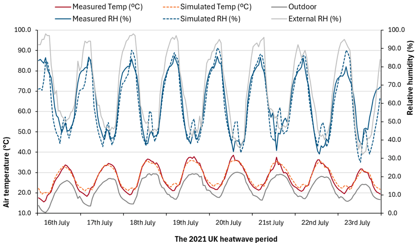
Fig. A1. Comparison between the simulations and measurements during the whole 2021 UK Heatwave period between the 16th and 23rd July 2021.
