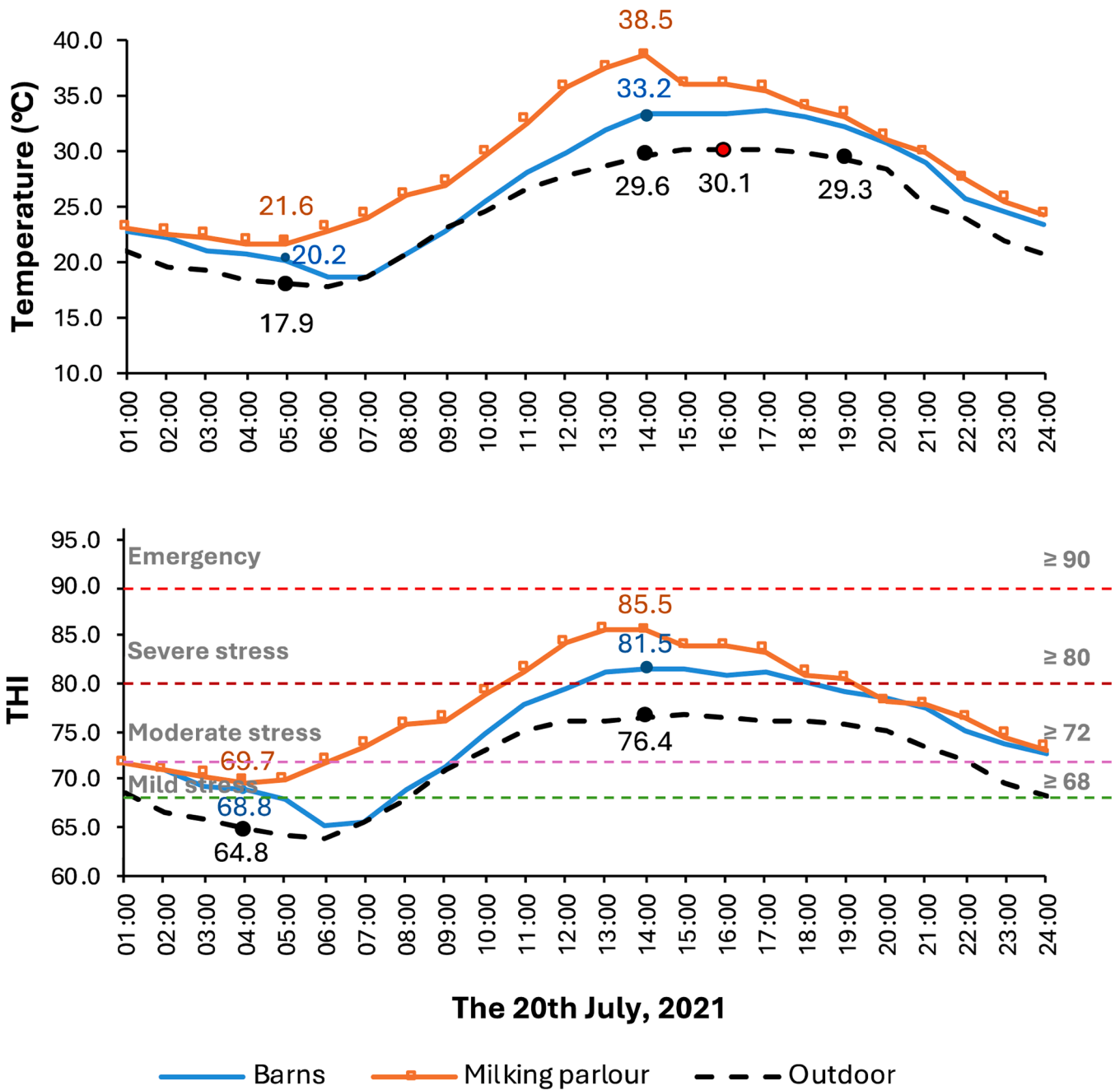
Fig. 8. Indoor temperature and Temperature-Humidity Index (THI) measurements for the cubicle yards and milking parlour on the hottest day of the 2021 UK heatwave.
