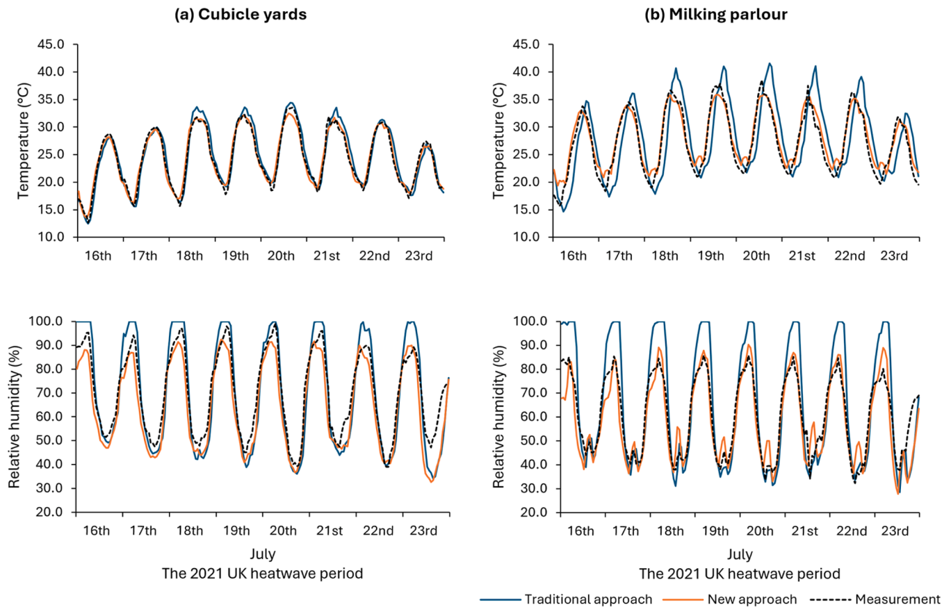
Fig. 5. Comparison of model accuracy between the traditional and new approaches. The new approach integrates a more realistic representation of latent and sensible heat dissipation from dairy cows.
