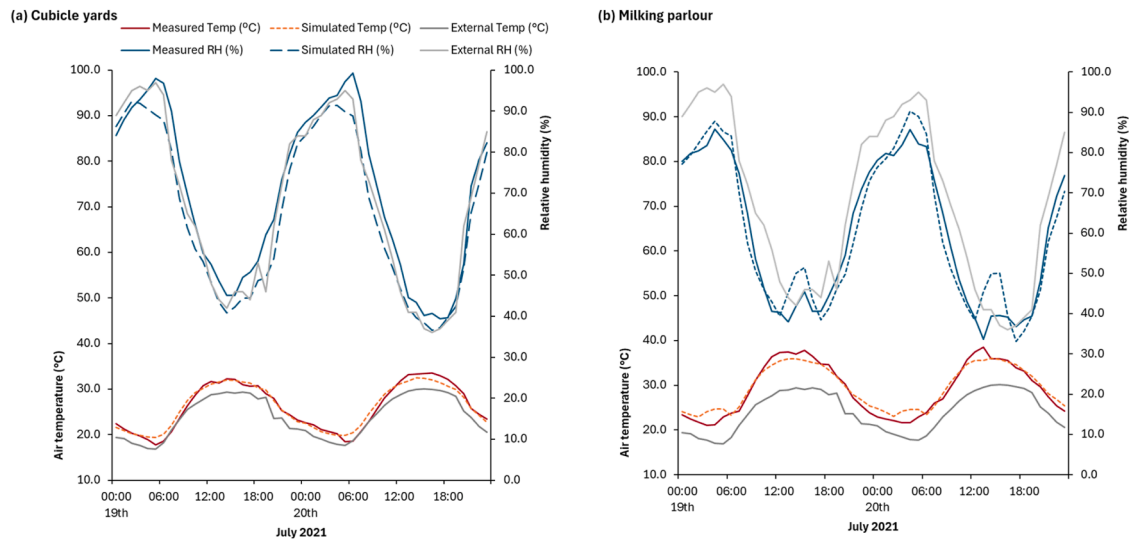
Fig. 6. Comparison of the measured and simulated temperature ( ^{\circ}\text{C} ) and relative humidity (%) data for the (a) cubicle yards and (b) milking parlour during the UK heatwave period between the 19th and 20th July 2021.
