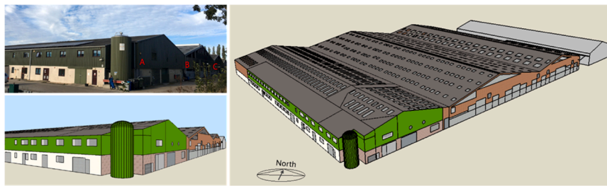
Fig. 2. Images of both the actual dairy cattle building and its basic thermal model created using DesignBuilder. The barn with the grey colour was newly built and unoccupied during that period.
