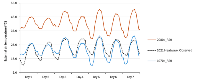
Fig. 4. Comparison between the observed 2021 heatwave and the synthetic heatwaves (Extreme Example Weeks) for the 1970s and 2080s with a return period of R = 20 years.
