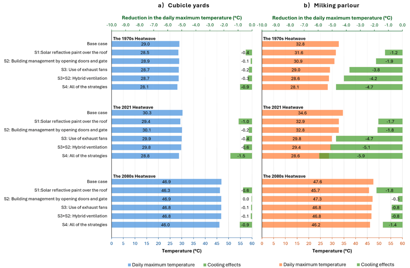
Fig. 13. Comparison of mitigation strategies based on the daily maximum temperature ( T_{daily}^{max} ) and their cooling effects, i.e., reduction in T_{daily}^{max} in the cubicle yards throughout the day and in the milking parlour during the milking periods: 04:00 – 06:50 and 14:00 – 16:30.
