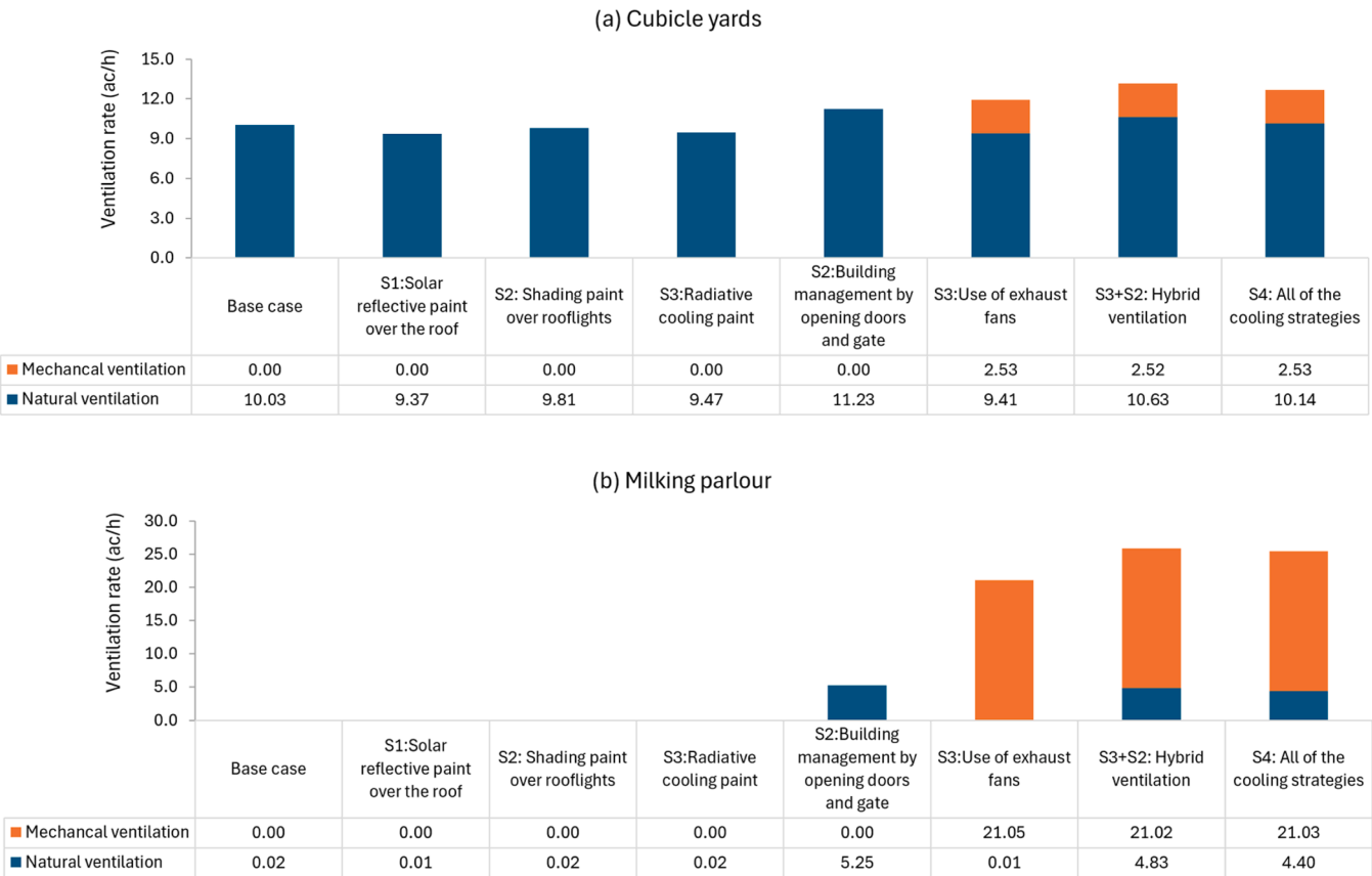
Fig. A2. The mean ventilation rate (ac/h) for the cubicle yards and milking parlour on 20th July 2021 under the heat stress mitigation strategies.
