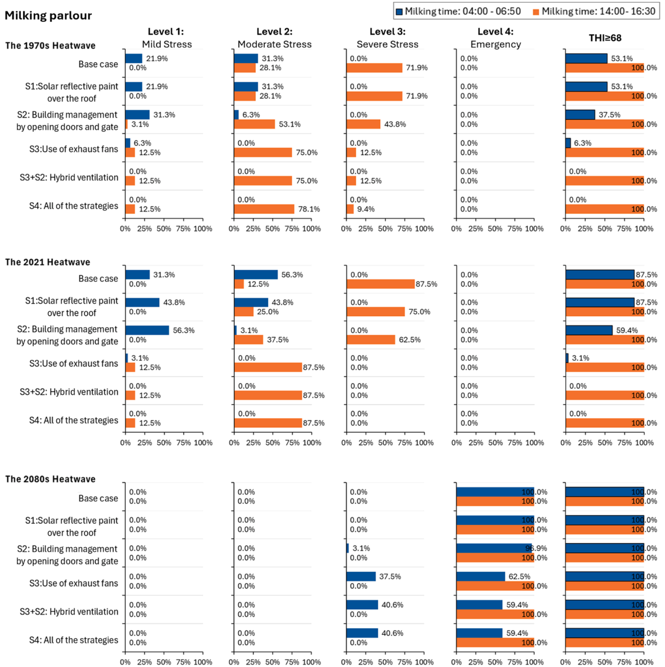
Fig. 15. Effects of mitigation strategies on Heat Stress Risk (%) and its distribution across heat stress levels during two milking periods: 04:00–06:50 and 14:00–16:30.
