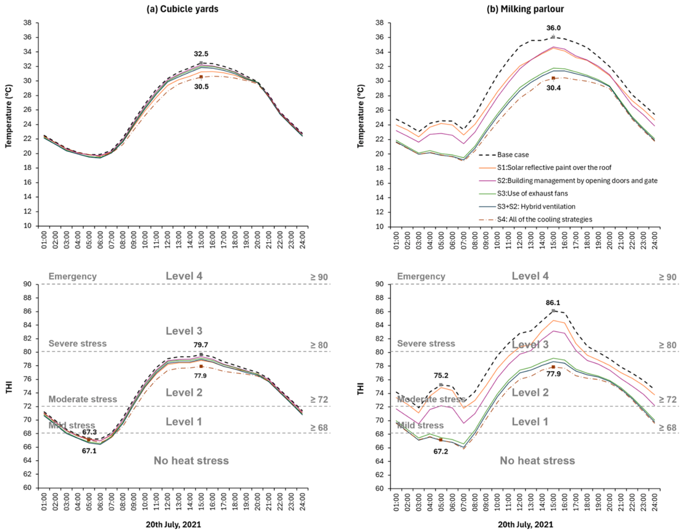
Fig. 10. The effects of heat stress mitigation strategies on the cubicle yards and milking parlour during the hottest day of the 2021 UK heatwave.
