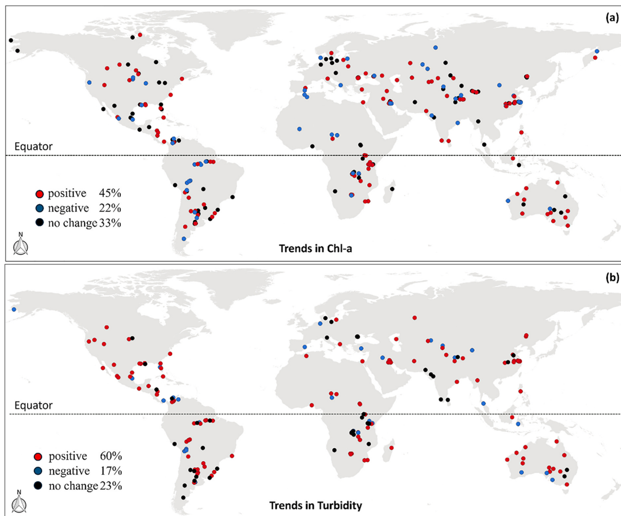
Fig. 3. Maps depicting de-seasonalized trends in (a) chlorophyll-a (Chl-a) and (b) turbidity, among CCI shallow lakes from 2002 to 2020. Red = significant positive trend ( p -value <0.05 ); blue = significant negative trend ( p -value <0.05 ); black = not significant trend ( p -value >0.05 ).
