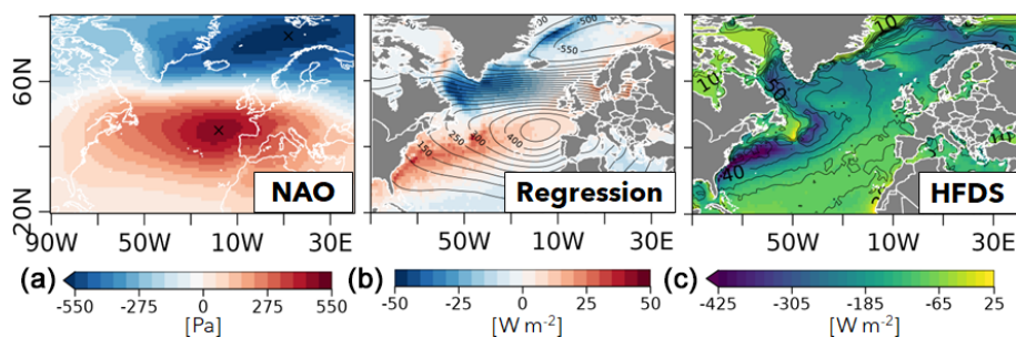
Figure A6. (a) Spatial pattern of the NAO in the ERA5 reanalysis, computed as in Fig. 7. (b) Regression map of the NAO index onto the DJF net surface heat fluxes in the ERA5 reanalysis. (c) Climatological DJF net surface fluxes in the ERA5 reanalyses.
