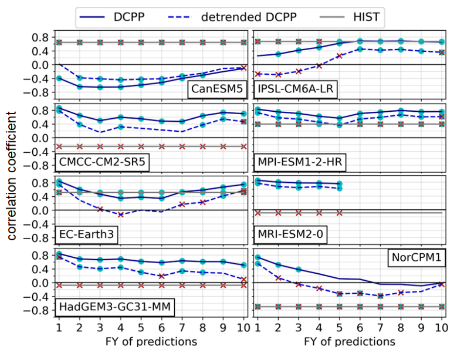
Figure 5. ACC of the spatially averaged OHC700 in the Labrador Sea (red box in Fig. 2) as a function of FY. Skill values are shown for the DCP (blue lines) and HIST (grey lines) ensembles and are evaluated against EN4. In DCP, skill is also computed after detrending both the forecast anomalies and the EN4 anomalies (detrended DCP; dashed blue lines). Cyan dots indicate ACC values that are significantly different from zero at the 95 % confidence level. Red crosses indicate that the HIST or the detrended DCP ACC values are significantly different from the DCP values. We note that ACC values are constant for HIST at all forecast years, since the evaluation period is fixed for their computation.
