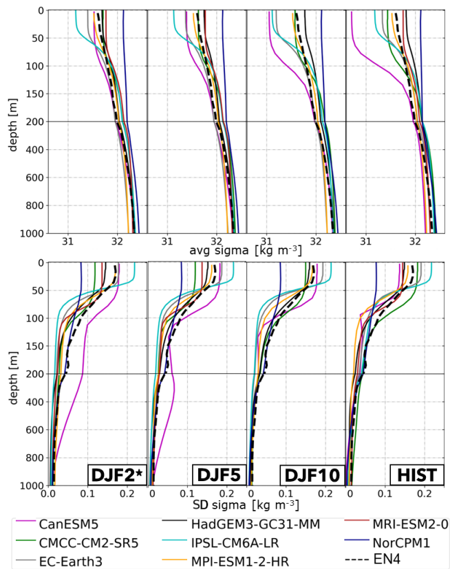
Figure 6. Top: mean-state climatology of the spatially averaged LS potential density anomaly in DJF (referred to 1000 m; \sigma_1 ) as a function of depth. The observational reference EN4 is included as a dashed black line. From left to right, it shows the results for the DCP (in forecast winters DJF2, DJF5, and DJF10) and HIST (in DJF) ensembles over the period 1970–2014. Bottom: the same as in the top row but for the standard deviation in time of the spatially averaged LS potential density anomaly.
