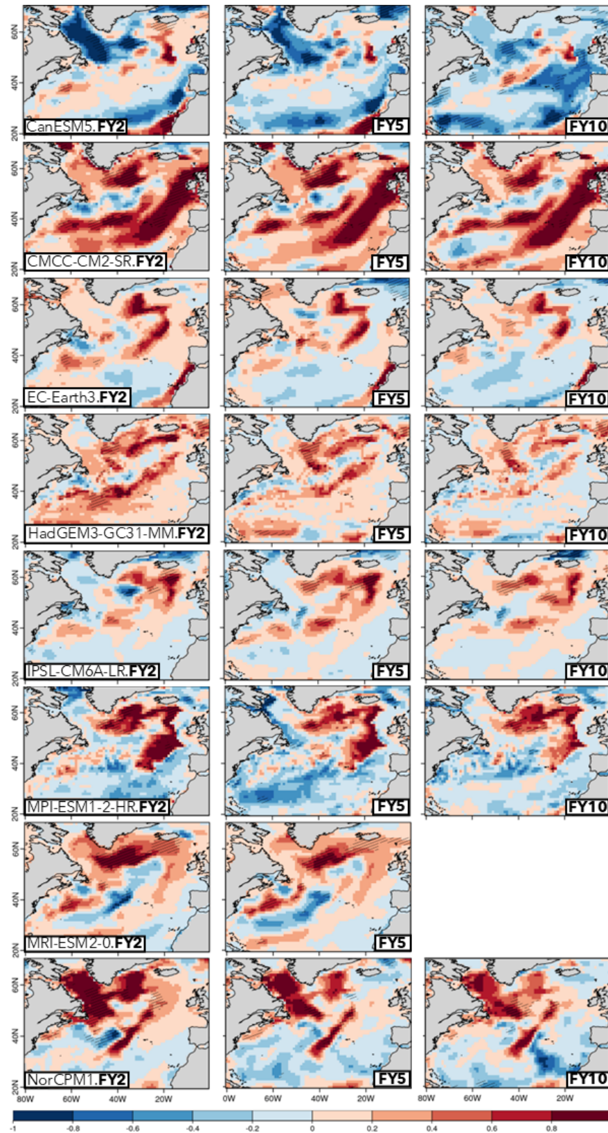
Figure A2. The same as in Fig. 1 but for the difference in ACC values between the DCP and HIST ensembles.
