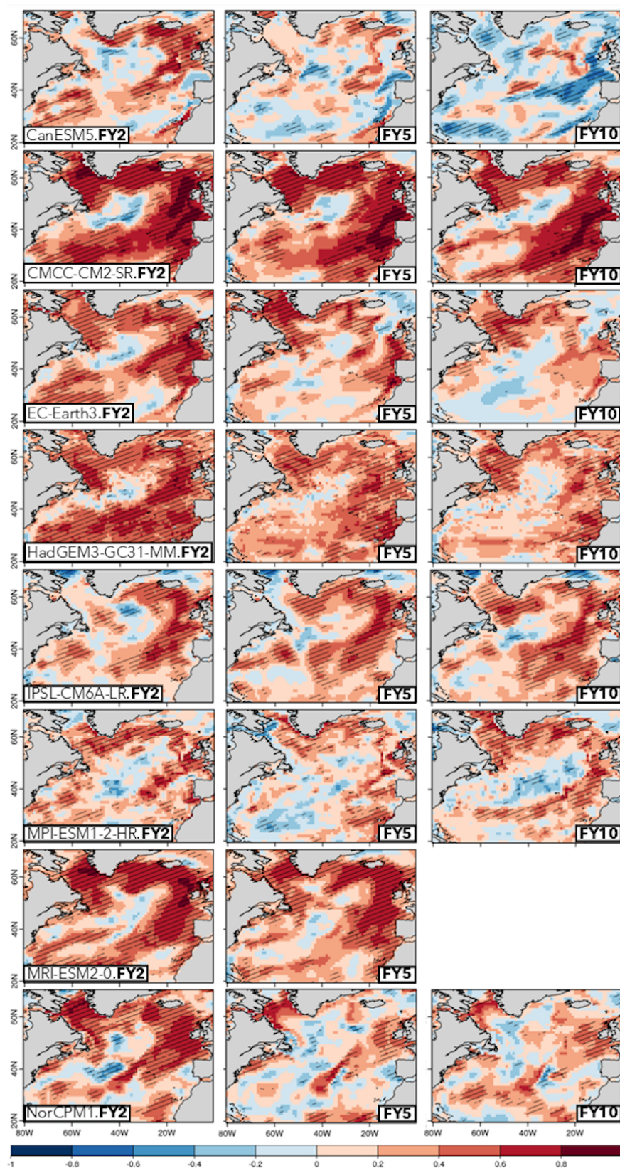
Figure A3. The same as in Fig. 1 but for the residual correlations in each DCPD ensemble.
