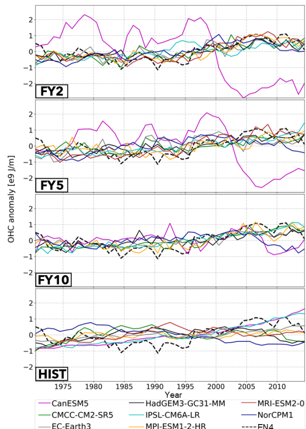
Figure 3. Time series of the spatially averaged OHC700 anomalies in the Labrador Sea region (red box in Fig. 2), for the DCPP (forecast years 2, 5, and 10) and HIST ensembles. The corresponding time series for EN4 observations is added as a dashed line.
