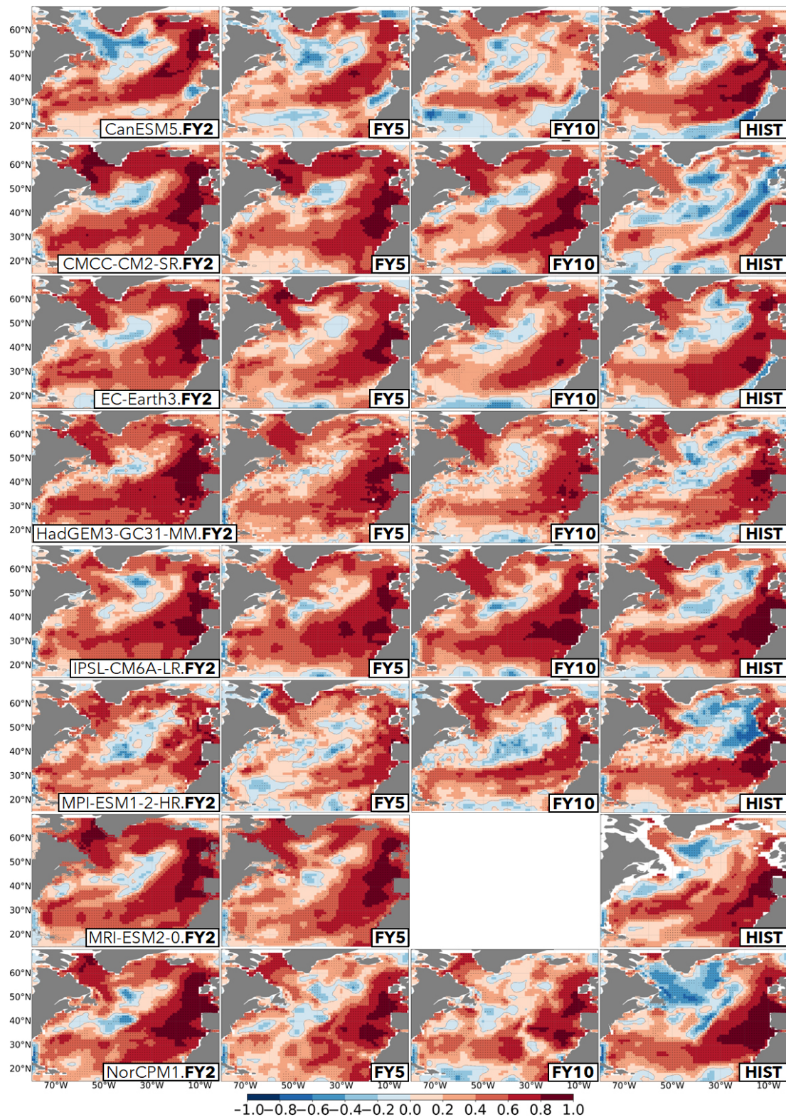
Figure 1. ACC maps for the OHC700 in the DCPP (forecast years 2, 5, and 10; columns 1–3, respectively) and HIST ensembles (column 4). Stippling indicates cells with correlation values statistically significant at the 95 % confidence level. All ACC values are evaluated against EN4 for the period 1970–2014. Each row shows the results for a different model.
