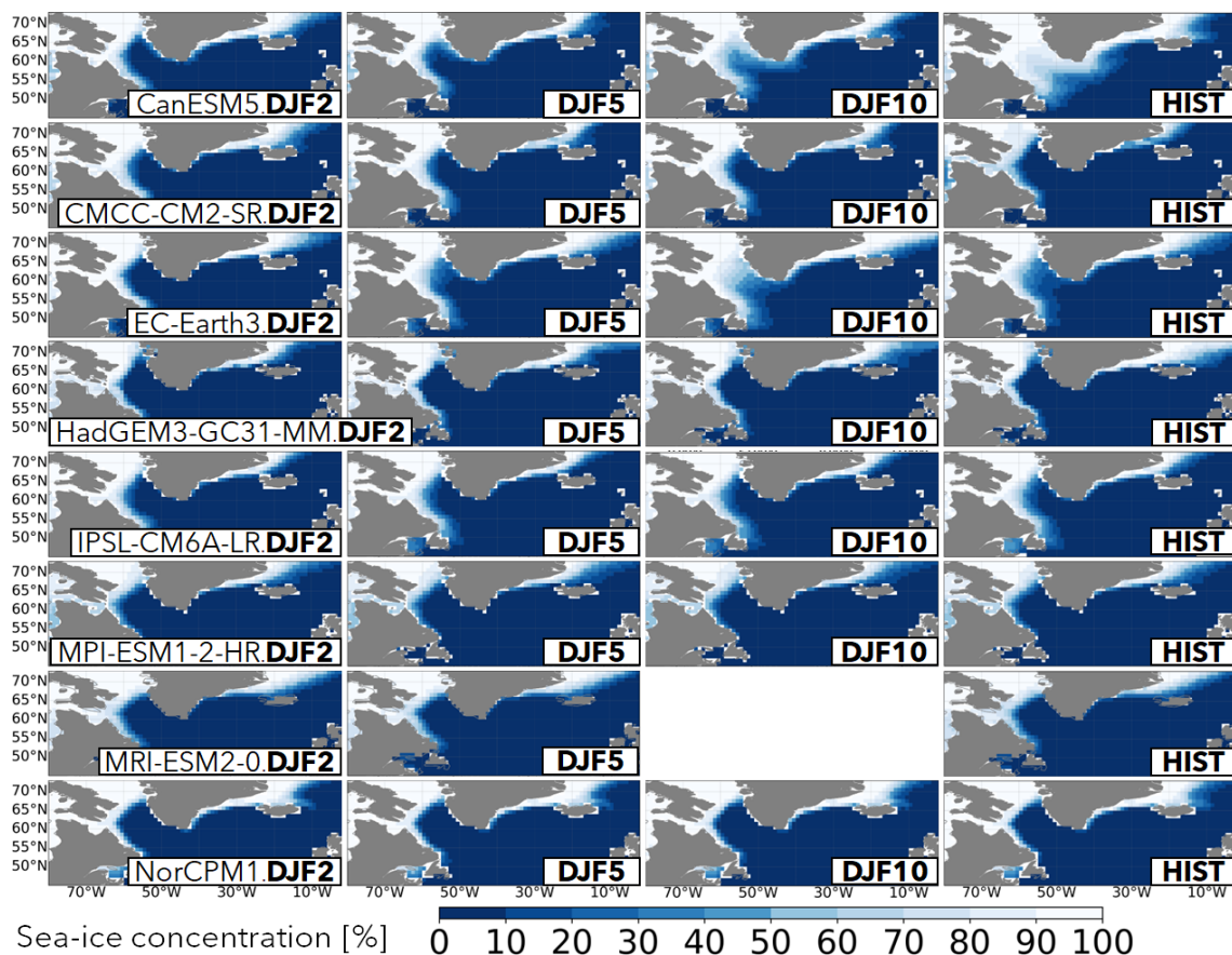
Figure A7. Sea ice concentration ( siconc ) maps for the initialized predictions for the forecast winters DJF2, DJF5, and DJF10 (columns 1–3, respectively) and for DJF in the HIST ensemble (column 4).
