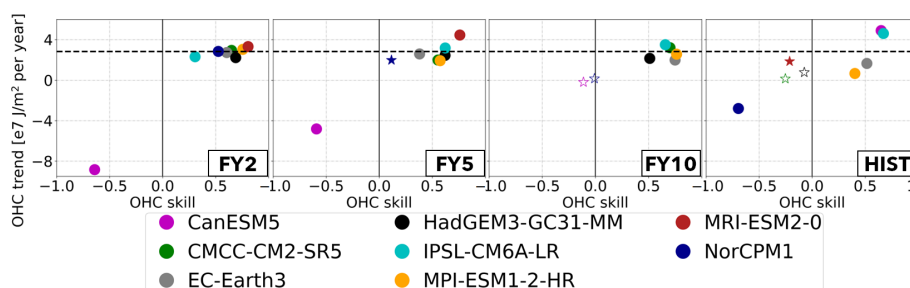
Figure 4. Scatter plot of the relationship between the skill of OHC in the Labrador Sea region (red box in Fig. 2) and the local OHC700 trend in both the DCP (forecast years 2, 5, and 10; columns 1–3, respectively) and HIST ensembles (column 4), all based on yearly averages. All trends were computed for the period of interest, 1970–2014 (see Sect. 2.4 for more information). Stars represent non-significant correlation values at the 95 % confidence level. Empty symbols represent non-significant trend values at the 95 % confidence level. The dashed black horizontal line represents the trends for EN4 observations.
