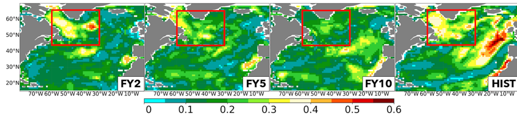
Figure 2. Standard deviation across models of the ACC values for OHC700 in DCPP (forecast years 2, 5, and 10; columns 1–3, respectively) and HIST ensembles (column 4). The red box encloses the Labrador Sea region, chosen to compute all area-weighted averages mentioned hereinafter, with boundary coordinates 45–65° N and 60–30° W.
