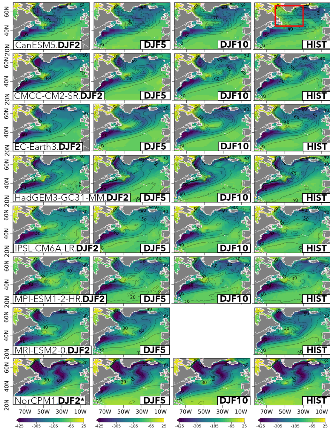
Figure A5. Climatological DJF net surface heat fluxes for the DCCP (in forecast winters DJF2, DJF5, and DJF10; columns 1–3, respectively) and HIST ensembles (in DJF; column 4). Negative (positive) values represent upward (downward) heat fluxes (in \text{W m}^{-2} ). The contour lines represent the associated standard deviation in time for the period 1970–2014. The red box in the upper-right plot depicts the LS region used in the analyses.
