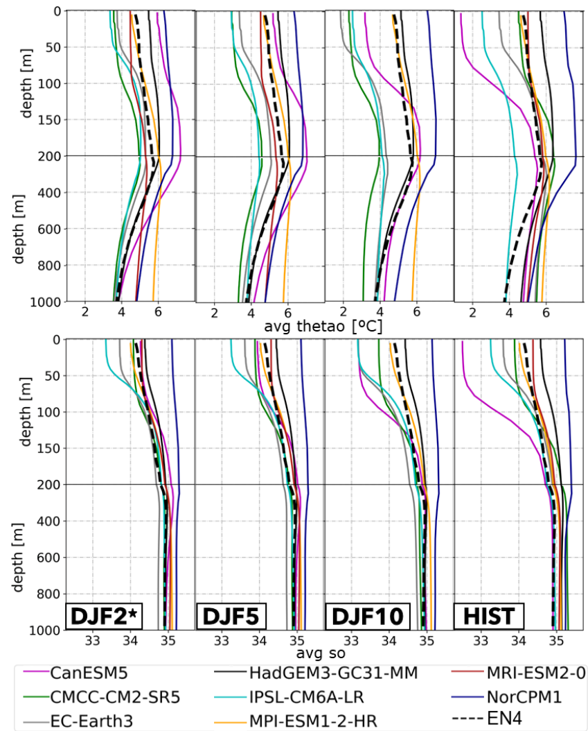
Figure A4. As in Fig. 6 but for the climatological vertical profiles of potential temperature (top) and salinity (bottom).
