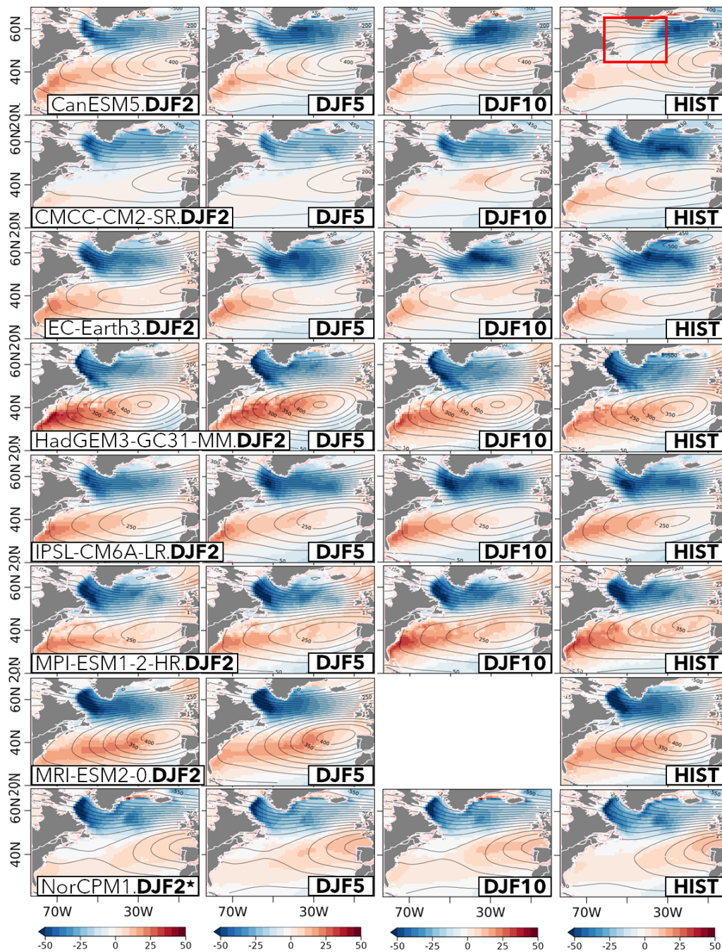
Figure 9. Regression maps of the NAO index onto net surface heat fluxes ( hfds ) for the DCP (in forecast winters DJF2, DJF5, and DJF10; columns 1–3, respectively) and HIST ensembles (in DJF; column 4). Negative (positive) values represent upward (downward) heat fluxes (in \text{W m}^{-2} ). The contour lines represent the corresponding NAO pattern. The red box in the upper-right plot depicts the LS region used in the analyses.
