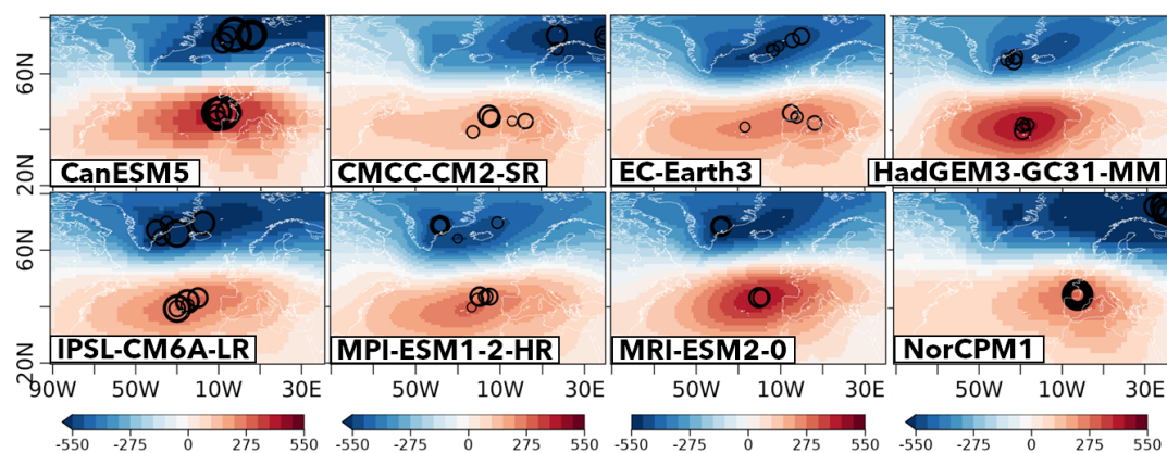
Figure 8. Same as in Fig. 7 but for DCPD experiments. In this case, the colour shading represents the NAO pattern at DJF2, and the circles (in increasing size) represent the centres of action of the ensemble mean for DJF2, 4, 6, 8, and 10, thus illustrating any potential shifts with forecast time.
