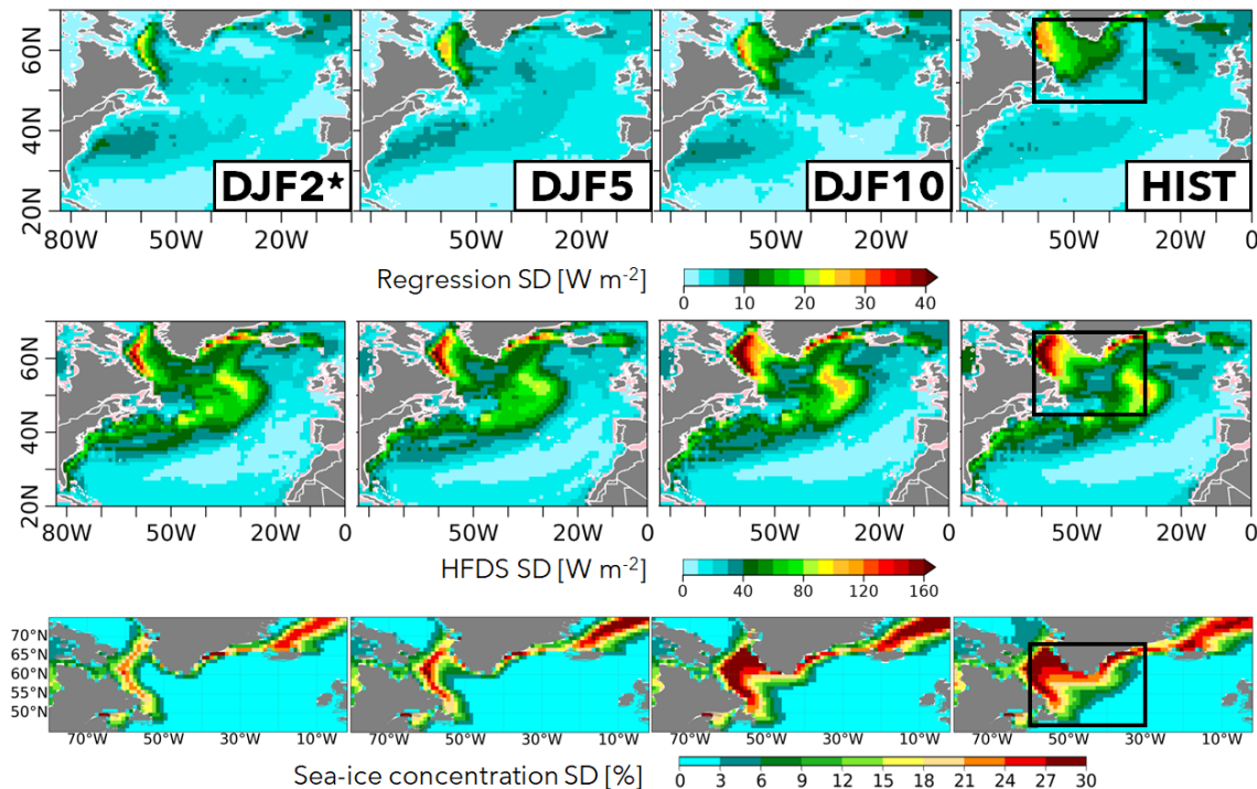
Figure 10. Top: inter-model spread for the regression coefficients in Fig. 9, as defined by the standard deviation across models. Middle: the same as above but for the climatological net surface heat fluxes in DJF. Bottom: the same as above but for the climatological sea ice concentration in DJF. The black box in the rightmost column depicts the LS region used in the analyses.
