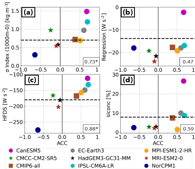
Figure 11. (a) Scatter plot of the relationship between the ACC skill in the Labrador Sea OHC700 and the climatological value of the index of the Labrador Sea density stratification in the HIST ensembles. The stratification index is computed as the density difference between 1000 m and the surface. The 1000 m level was chosen based on the visual inspection of the vertical profiles (Fig. 6) as a characteristic level of the mean properties of the ocean subsurface. Larger values of the index correspond to models where the LS is more stratified. Panel (b) is the same as panel (a) but between the ACC skill in the Labrador Sea OHC700 and the regressed values of the NAO index onto the Labrador Sea net surface heat fluxes in DJF. Panel (c) is the same as panel (a) but between the ACC skill in the Labrador Sea OHC700 and the climatological Labrador Sea net surface heat fluxes in DJF. Panel (d) is the same as panel (a) but between the ACC skill in the Labrador Sea OHC700 and climatological DJF sea ice concentrations in the Labrador Sea. In all panels, stars represent non-significant correlation values at the 95 % confidence level. The dashed black horizontal line represents the respective reference dataset: (a) EN4, (b, c) ERA5, and (d) HadISST. The linear relationship between the different pairs of metrics is measured with correlation values in the model space, shown for each plot in the lower-right corners, with asterisks indicating if the correlation coefficient is significant at the 95 % confidence level.
