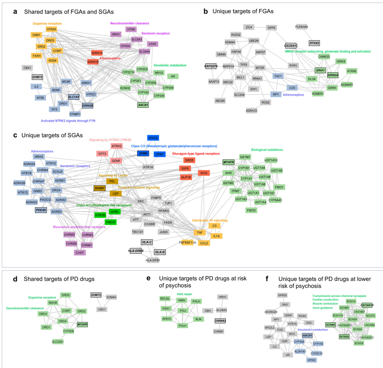
Fig. 5 FGA and SGA targets and targets of PD drugs at risk of psychosis and at lower risk of psychosis are involved in different network modules in the human interactome. The networks of the proteins targeted by a shared targets of FGAs and SGAs, b unique targets of FGAs, c unique targets of SGAs, d shared targets of PD drugs, e unique targets of PD drugs at risk of psychosis and f unique targets of PD drugs at lower risk of psychosis, were constructed using the STRING database. Network nodes represent proteins and edges represent protein-protein associations retrieved from the STRING database. The topological modules in these networks were identified using the MCL algorithm. The nodes in the topological modules enriched for specific biological processes have been denoted using separate colours. In a–c , genes shown in bold italics are unique SZ-associated genes (that are not associated with PD) found in the network. In d–f , genes shown in bold are unique PD-associated genes (that are not associated with SZ) and those shown in bold italics are unique SZ-associated genes (that are not associated with PD) found in the network.
