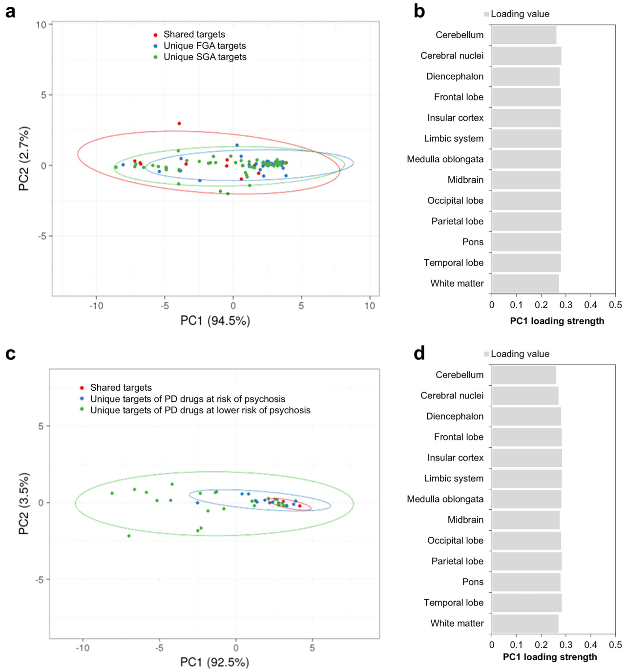
Fig. 2 Principal component analysis of the drug targets revealed their clustering into overlapping ellipses, albeit of differing expression variability in the brain. PCA was performed with the \log_2 -transformed probe intensities of the drug targets in 13 major brain areas in the microarray dataset of Allen Brain Atlas. A data matrix with brain regions (rows) and the drug targets (columns) was constructed out of these log-transformed values. Unit variance scaling was applied across this matrix for normalisation. Singular value decomposition with imputation was used to extract the principal components (PCs). In a , the component scores ( n = 93 ) corresponding to PC1 and PC2 explaining 94.5% and 2.7% of the total variance have been plotted along X and Y axes respectively. The three prediction ellipses correspond to the shared targets of FGAs and SGAs (red), the unique targets of FGAs (blue), and the unique targets of SGAs (green). The probability of a new data point from the same group falling within these ellipses is 0.95. In b , the loading strengths of the 13 dimensions, i.e., the brain regions, contributing to PC1, have been shown. In c , the component scores ( n = 38 ) corresponding to PC1 and PC2 explaining 92.5% and 3.5% of the total variance have been plotted along X and Y axes respectively. The three prediction ellipses correspond to the shared targets of the PD drugs irrespective of whether they induce psychosis or not (red), the unique targets of PD drugs at risk of psychosis (blue), and the unique targets of PD drugs at lower risk of psychosis (green). In d , the loading strengths of the brain regions contributing to PC1 have been shown.
