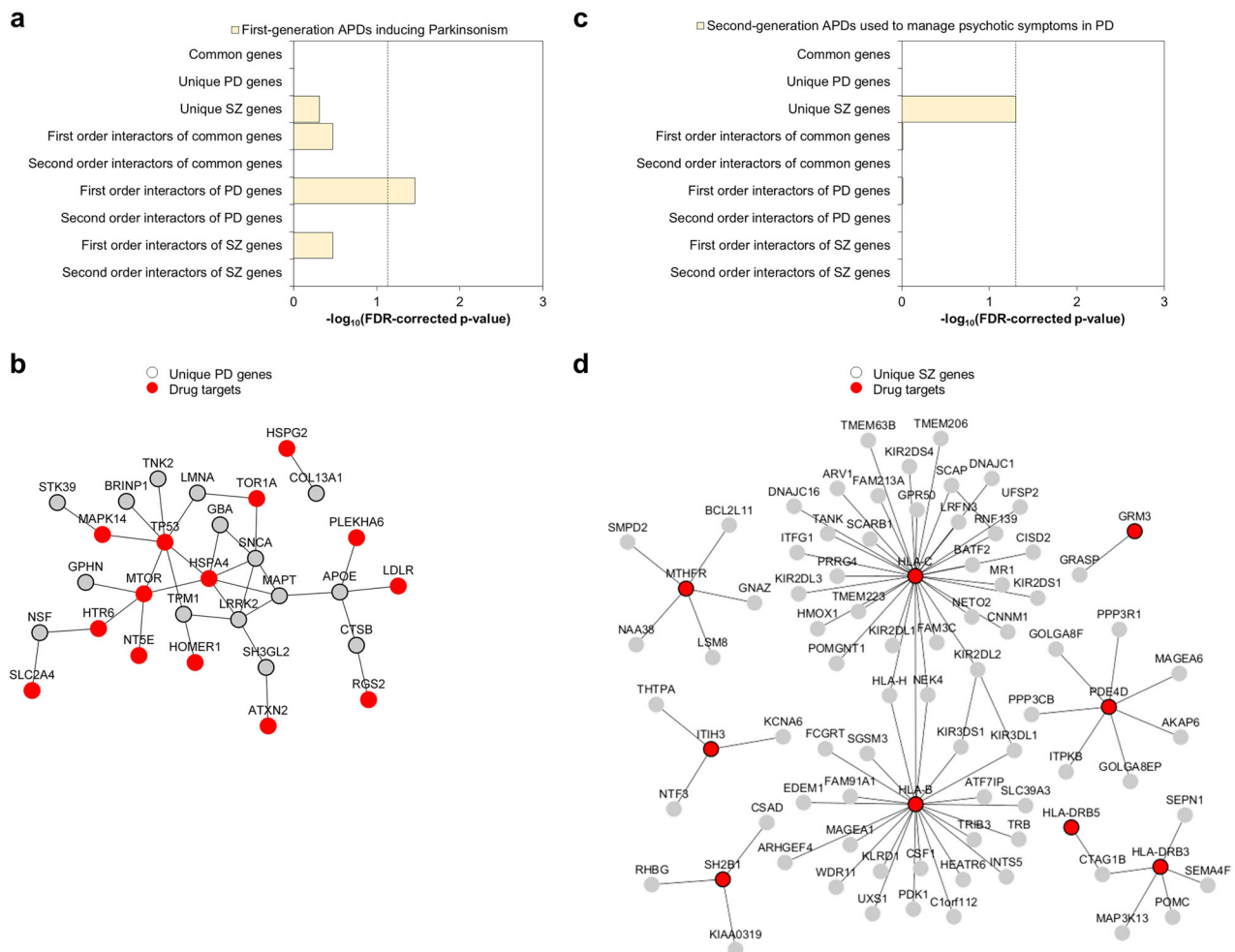
Fig. 6 The different effects of FGAs and SGAs could be attributed to their associations with PD and SZ-associated genes. The network proximity of FGA and SGA drug targets to genes associated exclusively with PD or SZ, as well as genes shared between the two disorders, were examined. Specifically, the enrichment of FGA and SGA targets among the following sets were assessed: unique PD genes, first-order interactors of unique PD genes in the interactome (i.e., their direct interactors), and second-order interactors of unique PD genes (i.e., genes interconnected to unique PD genes via an intermediate interactor, separated by two steps/interactions). Similar sets were assembled for unique SZ genes and shared PD/SZ genes. a and b show the exclusive enrichment of FGA targets for the first-order interactors of unique PD genes (direct interactors). c and d show the exclusive enrichment of SGA targets for the unique SZ genes themselves rather than their interactors. The bar graphs in a and c show the -\log_{10}(p\text{-value}) of enrichment after correction for multiple hypotheses using the Benjamini-Hochberg method. The network nodes in b and d represent proteins and edges represent protein-protein interactions.
