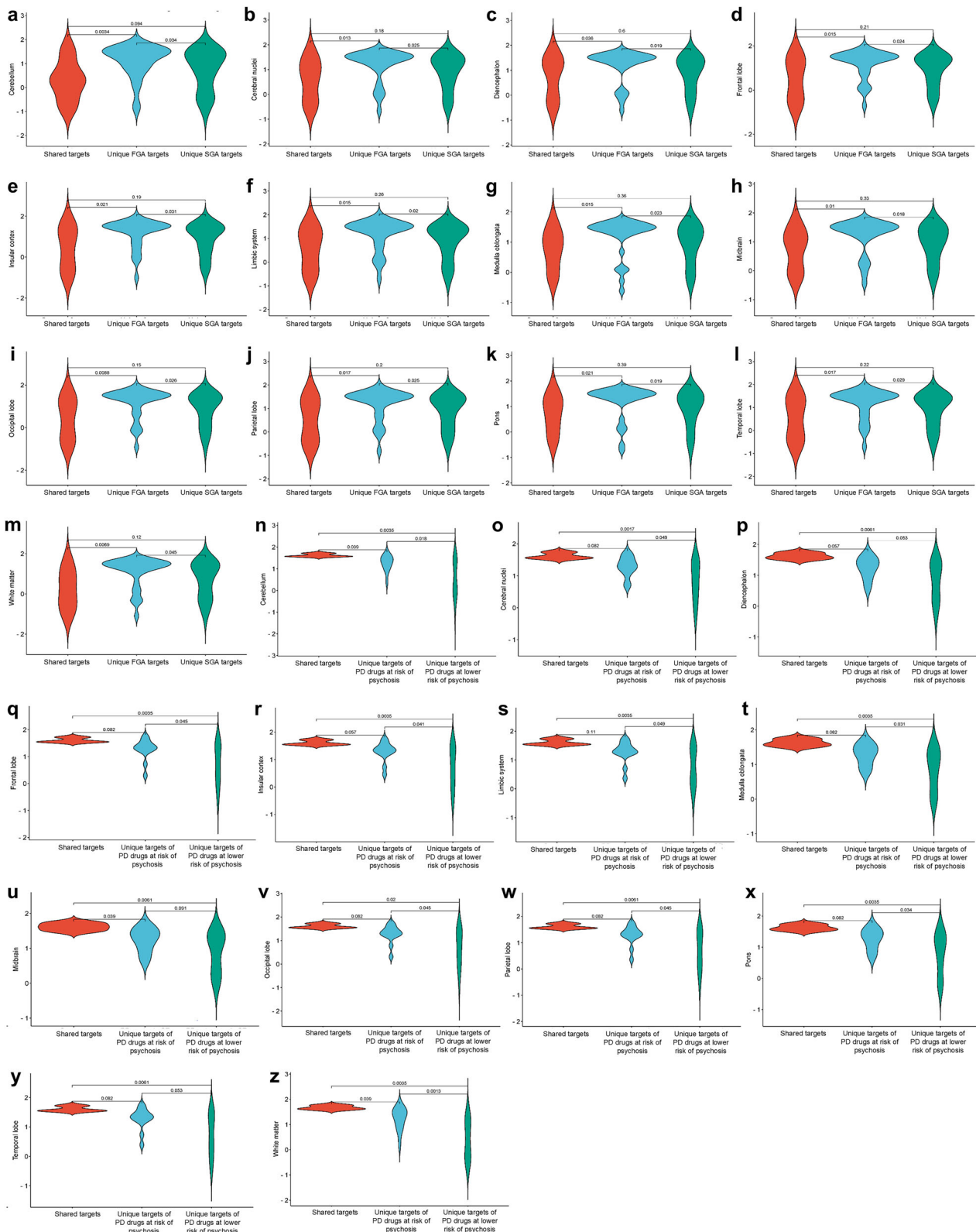
Fig. 3 The targets of FGAs and SGAs and PD drugs at risk (or not) of inducing psychosis exhibit differences in region-wise gene expression distributions. The varying average probe intensity distributions of the shared targets of FGAs and SGAs (red), the unique targets of FGAs (blue), and the unique targets of SGAs (green) in 13 major brain areas (see Y axes) have been shown using the violin plots in a–m . The varying average probe intensity distributions of the shared targets of PD drugs irrespective of whether they induce psychosis or not (red), the unique targets of PD drugs at risk of psychosis (blue), and the unique targets of PD drugs at lower risk of psychosis (green) in 13 major brain areas (see Y axes) have been shown using the violin plots in n–z . In a–z , the p -values denoting the statistical differences between pairs of drug target categories were computed using the Wilcoxon rank sum test and adjusted for multiple hypotheses using the Benjamini-Hochberg method.
