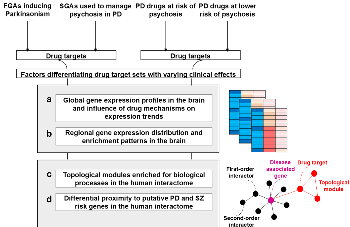
Fig. 1 Flow chart depicting the concepts examined in the study. Antipsychotic drugs exhibiting two distinct clinical effects were collected, specifically, first-generation antipsychotics (FGAs) causing Parkinsonism and second-generation antipsychotics (SGAs) used to manage psychotic symptoms in Parkinson's disease (PD). Similarly, PD drugs with two effects were compiled, those at risk of inducing psychosis and those at lower risk of psychosis. The genes targeted by these four drug categories were identified. Subsequently, we investigated four factors (a–d) that could potentially help differentiate the target sets of PD and antipsychotic drugs with varying clinical effects: a The global expression trends of the drug targets in the brain and the impact of the different neurotransmitter systems that the drugs regulate on these trends; b The regional variations in the expression levels of drug targets and their numerical overrepresentation among genes highly expressed in specific brain regions; c The topological modules formed by the drug targets in the human interactome and their enrichment for specific biological processes; d The proximity of the drug targets to genes associated with PD and SZ, as well as their first-order and second-order interactors.
