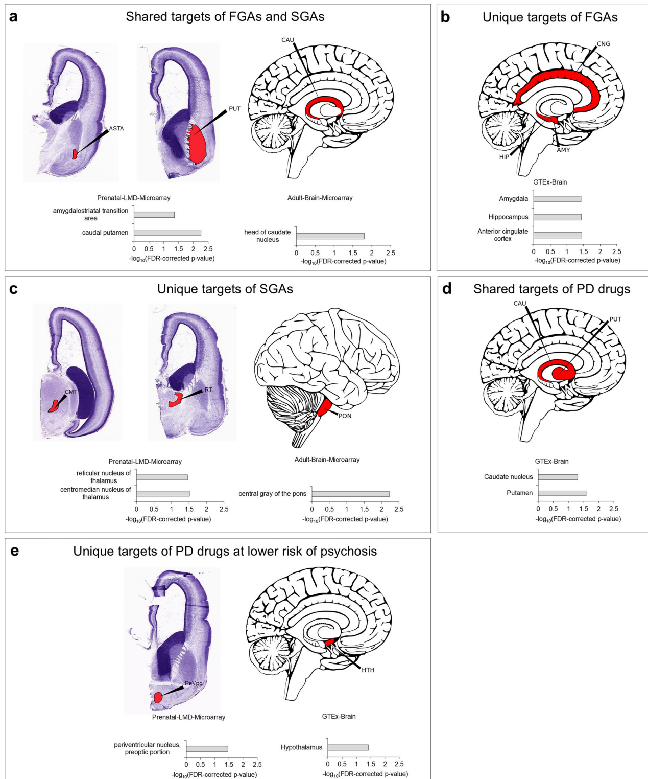
Fig. 4 Antipsychotic and PD drug targets showed differential enrichment patterns in specific brain regions. The enrichment of the drug targets for genes showing high expression in specific regions extracted during prenatal stages (LMD microarray dataset), from adults (Allen Brain Atlas microarray and GTEx RNA-sequencing datasets), and during prenatal and adult stages (Allen Brain Atlas developmental transcriptome RNA-sequencing dataset), was examined. a–c show the specific areas in which the shared and unique targets of SGAs and FGAs are highly expressed, with the adult areas marked in brain maps and the prenatal areas highlighted against the background of Nissl-stained brain sections (Interactive Atlas Viewer, Allen Brain Atlas). d and e show the specific areas in which the shared targets of PD drugs and the unique targets of PD drugs at lower risk of psychosis are highly expressed. The accompanying bar graphs show the -\log_{10}(p\text{-value}) of enrichment after correction for multiple hypotheses using the Benjamini-Hochberg method. Note that the specific regions that showed enrichment at p\text{-value} < 0.05 after correction (i.e., -\log_{10}(p\text{-value}) > 1.30103 ) are shown in the brain maps and Nissl-stained brain sections.
