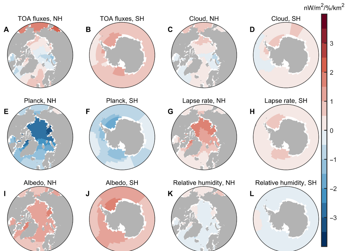
Fig. 4. Sensitivity of global TOA radiation to regional SIC reduction and its breakdown into contributions from individual radiative processes. (A and B) Response of annual mean global TOA radiation to regional SIC reduction in unit surface area ( -\partial R/\partial SIC , calculated with Eq. 4). (C and D) Contribution of cloud changes. (E and F) Contribution of vertically uniform temperature changes (Planck feedback). (G and H) Contribution of vertically nonuniform temperature changes (lapse rate feedback). (I and J) Contribution of surface albedo changes. (K and L) Contribution of RH changes. A positive value at a given location indicates that sea ice loss at that location leads to a radiative heating of the climate system, averaged annually and over the globe. Seasonal values and regional responses are shown in figs. S10 to S12.
