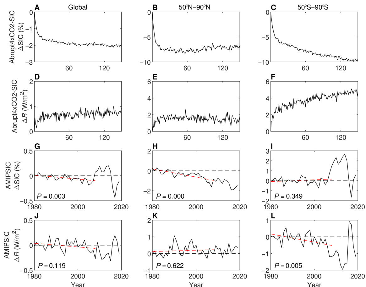
Fig. 1. SIC changes and corresponding radiative effects under CO 2 -induced global warming and during the historical period of 1980–2019. (A to F) Results from the abrupt4xCO 2 -SIC experiments, where the changes are relative to the first year of the experiment. (G to L) Results from the AMIPSIC experiments, where the changes are calculated relative to the average value between 1980 and 1989. The red dashed lines denote the trends over 1980–2008, and the P values of t tests for these trends are shown in each panel. The black dashed lines are base lines.
