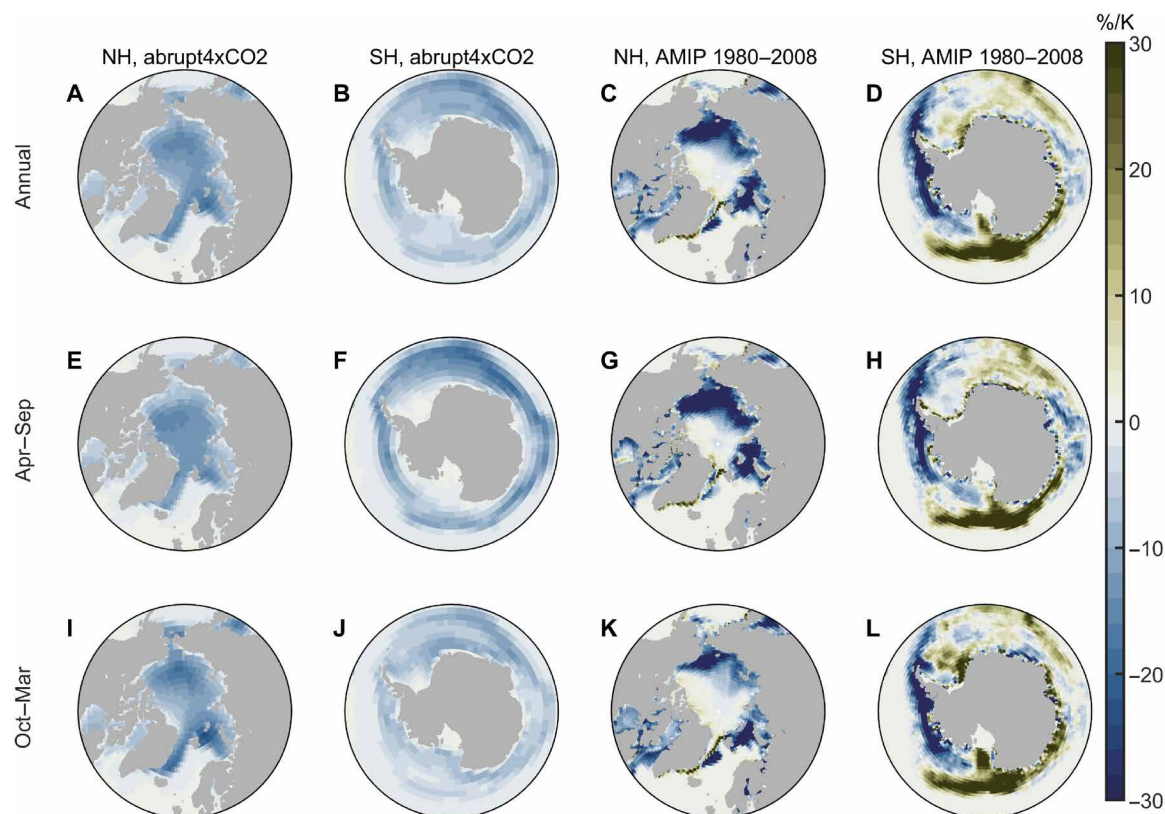
Fig. 2. Change of SIC normalized by the change of global mean surface temperature. (A and B) Annual SIC change pattern in abrupt4xCO 2 experiments, calculated using the differences between average value of the piControl experiments and years 131 to 150 of the abrupt4xCO 2 experiments (table S1). (C and D) Historical annual SIC change pattern during 1980–2008 (AMIP SIC). (E to H) SIC change patterns in April to September. (I to L) SIC change patterns in October to March.
