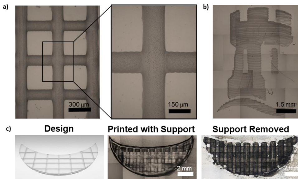
Fig. 4. Structures fabricated via inkjet based 3D printing from the lead candidate material, polymer 32: a) square mesh structure; b) inkjet printed castle logo of University of Nottingham; c) cartilage patch scaffold containing through channels achieved by co-printing with water soluble support materials.
