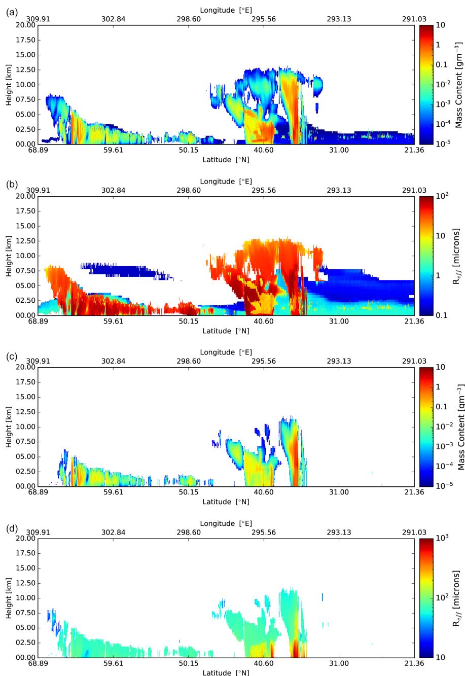
Figure 7. Panels (a) and (b) correspond to the total hydrometer and aerosol mass density and the effective particle radius. Panels (c) and (d) correspond to the mass and effective radius for (solid+liquid) precipitation. More detailed species-by-species information can be found in Qu et al. (2022).
