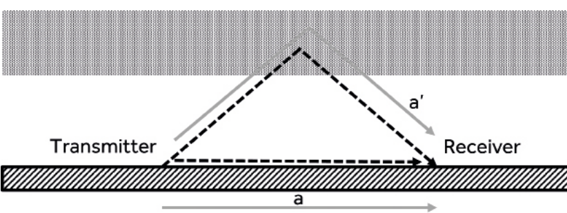
5 The geometry of Appleton's experiment. The direct wave along the ground would travel a distance, a , to the receiver, while the indirect wave would travel a greater distance, a' . By changing the wavelength of the carrier signal slowly throughout the experiment, Appleton was able to estimate the path difference ( a'-a ) from the number of signal maxima he observed. From this he was able to estimate the height of the reflecting layer to be 80–90km.
