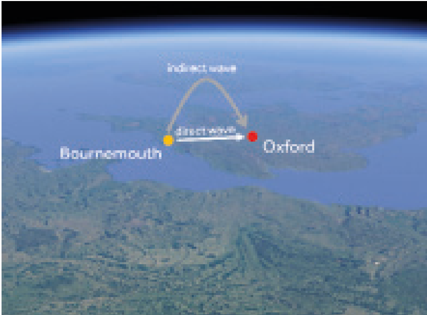
4 The scale of Appleton's experiment. A radio wave from BBC Bournemouth was received at Oxford, 140km away. This path was sufficiently short that both a 'direct' wave along the ground and an 'indirect' wave via the upper atmosphere would both arrive at the receiver. Appleton interpreted the fading of such radio signals as destructive interference caused by the phase difference resulting from the different paths the two waves. (Google Earth, using data from Landsat/Copernicus, Data SIO and NOAA)
