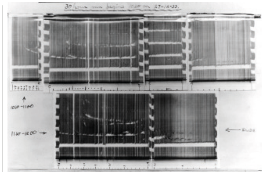
8 An example of an early ionospheric sounding from 1933. Photographic paper was fed past a slit in front of an oscilloscope on which the ground and ionospheric echoes were displayed for a given frequency. By moving the paper and changing the frequency of the radio pulse, a plot of time-of-flight (proportional to height) against frequency (proportional to the square-root of the electron concentration) was generated. In these early plots, frequency increases from right to left. (Ditton Park Archive at the UK Solar System Data Centre)
