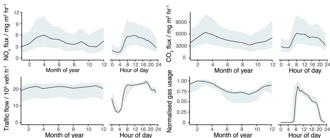
Figure 3. Median average monthly and diel profiles for \text{NO}_x flux, \text{CO}_2 flux, traffic flow and natural gas usage (2021–2023). The gas usage monthly profile uses data from the North Thames LDZ which includes central London consumption. Since gas usage data has a maximum resolution of 24 h, a diel consumption profile was estimated from activity factors as discussed in the text. These are both normalized for presentation on the same axis. Shaded regions span the interquartile range (IQR) of the averaging.
