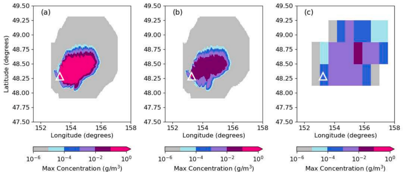
Fig. 4. Plan view of maximum ash concentration in (a) ATHAM simulation (fine ash particles scaled so that the time-integrated fine ash mass matches the time-integrated mass in InTEM as in Fig. 3(a)), (b) ATHAM simulation (fine ash only, scaled so that the time-integrated fine ash mass matches the time-integrated mass in InTEM as in Fig. 3(b)) and (c) NAME-InTEM simulation using the effective source determined using InTEM (Fig. 2c) and at the same time as Fig. 3.
