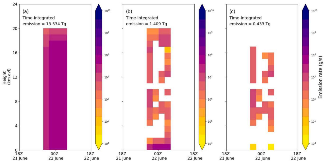
Fig. 2. (a) Prior mean effective emission profile with a uniform vertical ash distribution, (b) optimal posterior time-height effective emission profile determined by InTEM using ash only satellite retrievals (c) optimal posterior time-height effective emission profile determined by InTEM using ash and clear sky satellite retrievals, for phase 7 of the Raikoke eruption. Note the log scale used for the release rate.
