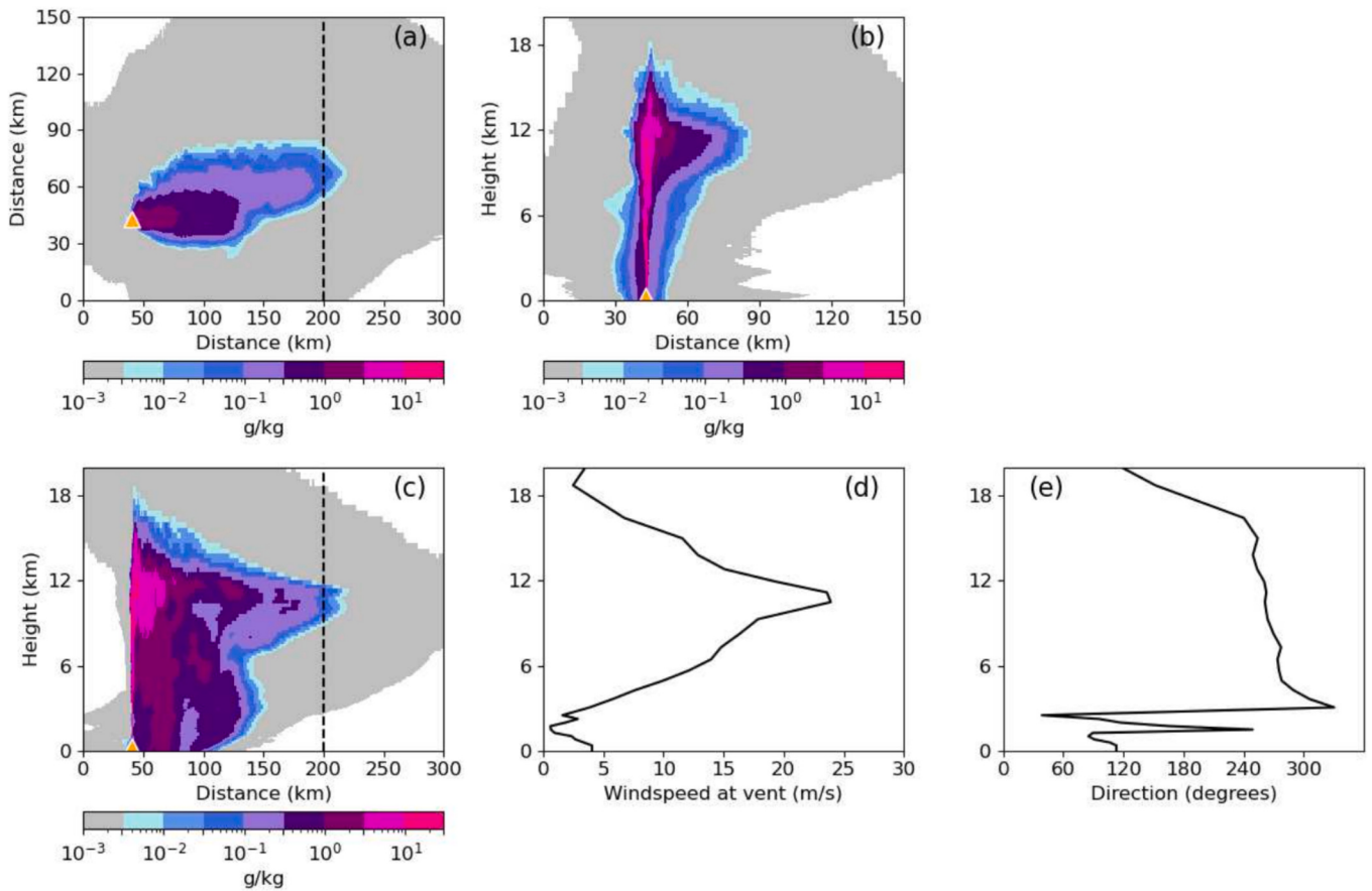
Fig. 1. (a) Plan view of the vertically averaged ash plume (x-axis is distance to the East and the y-axis is the distance to the north) (b) Mean North-South cross section through the ash plume (c) Mean East-West cross section through the ash plume, both at the volcano vent location at 120 min into the ATHAM simulation of phase 7 of the Raikoke eruption. (d) Vertical profile of wind speed and (e) vertical profile of wind direction prescribed in the simulation. Note that the heights here are asl and the dashed black line in panels (a) and (c) indicates 150 km downwind from the volcano vent.
