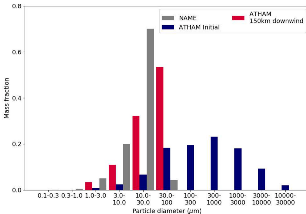
Fig. 5. Effective particle size distribution (PSD) used in NAME (grey), total PSD at the volcano vent in ATHAM (navy) and total PSD 150 km from the volcano vent in the ATHAM simulation (red). (For interpretation of the references to colour in this figure legend, the reader is referred to the web version of this article.)
