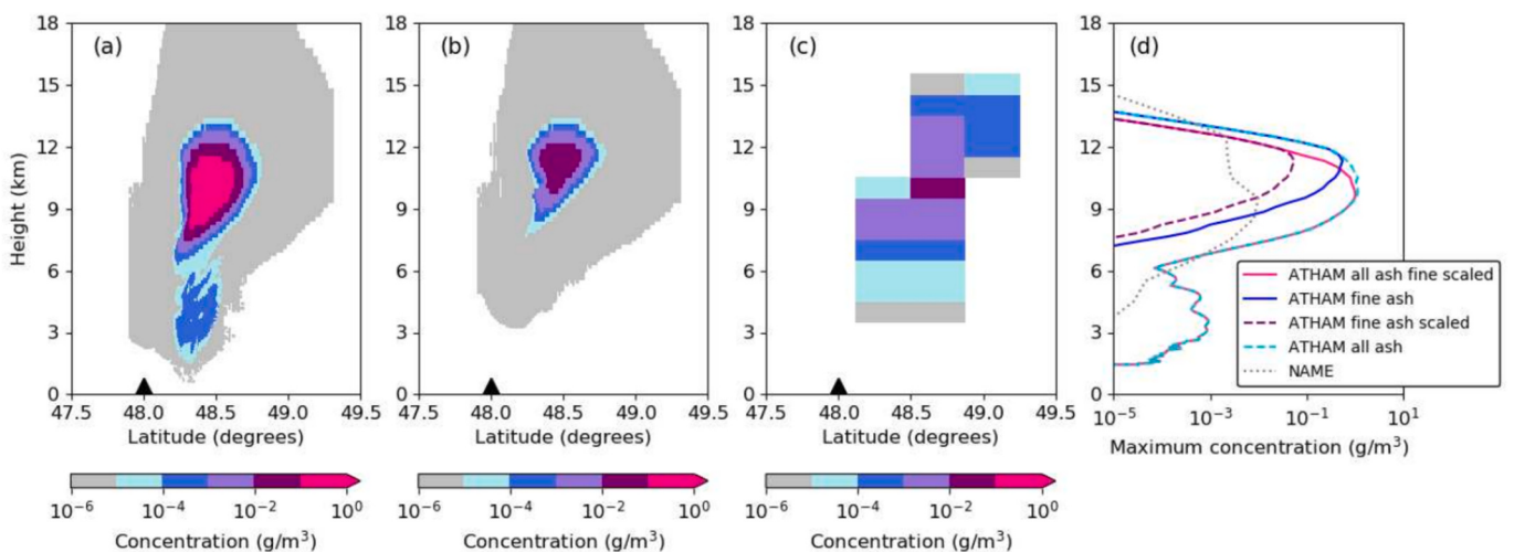
Fig. 3. Vertical cross section of ash concentration through the ash cloud 150 km downwind from the volcano vent at 155.9^\circ E in (a) ATHAM (all ash with fine ash particle sizes scaled so that the time-integrated fine ash mass emitted, TE_0 , matches the time-integrated mass emitted in InTEM), (b) ATHAM (fine ash only, scaled so that the TE_0 matches the time-integrated mass emitted in InTEM) and (c) NAME-InTEM simulation using the effective source determined using InTEM (Fig. 2c). (d) shows the vertical profile of the maximum concentration for the NAME-InTEM simulation (grey dotted), scaled-ATHAM simulation (fine ash only as in (b), purple dashed line) and unscaled-ATHAM simulation (fine ash only, blue line), scaled-ATHAM simulation (all ash with fine ash scaled as in (a), pink line) and unscaled-ATHAM simulation (all ash, cyan dashed). Note the logarithmic scale on the x-axis. (For interpretation of the references to colour in this figure legend, the reader is referred to the web version of this article.)
