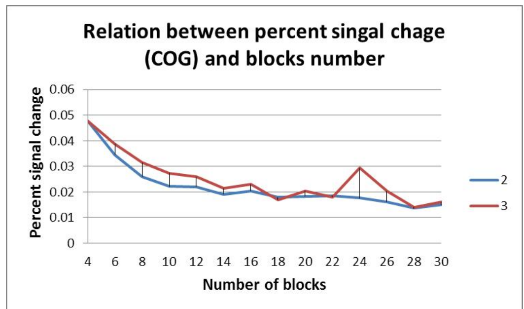
Fig. 9. The relationship between percent signal change of COG in left SPL or left precentral gyrus and the number of blocks. In the graph, curve 2 represents the left SPL whereas curve 3 denotes the left precentral gyrus. Abbreviation: COG, center of gravity.
