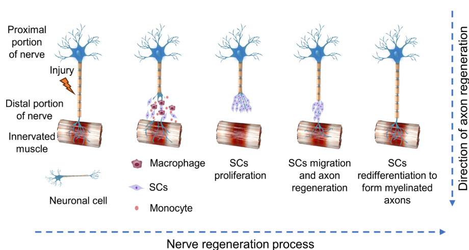
Figure 1: The regeneration mechanism of peripheral nerve injuries.
