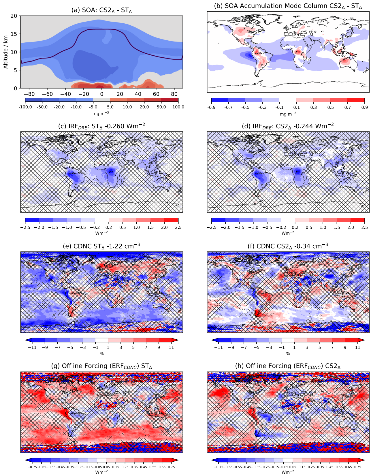
Fig. 4 | Secondary organic aerosol (SOA) changes, aerosol scattering forcing, cloud droplet number concentration changes and associated cloud droplet forcing. Difference in (a) zonal mean SOA increase and (b) accumulation mode SOA column increase between CRI-Strat 2 ( CS_{2\Delta} ) and Strat-Trop ( ST_{\Delta} ). Radiative forcing from the change in the aerosol direct radiative effect ( IRF_{DRE} ) for (c) ST_{\Delta} and (d) CS_{2\Delta} . Percentage change in vertically averaged cloud droplet number concentration
