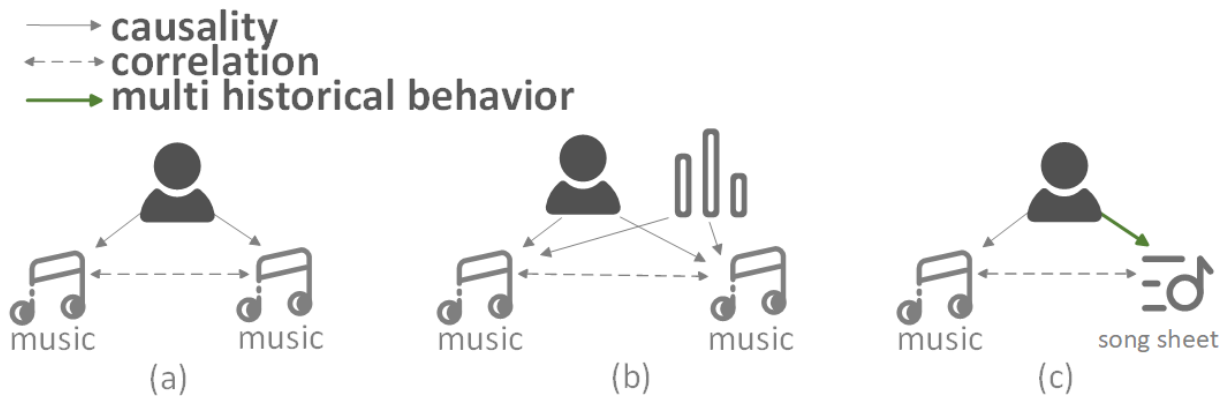
FIGURE 1. (a) The current SBRS generates recommendations by analyzing the co-occurrence patterns between users and music. (b) However, the reliance on co-occurrence between users and music can be misleading. For instance, a user's choice to listen to a specific song might not genuinely reflect an affinity for its genre but could be a result of recent exposure that has temporarily popularized the track. (c) In actuality, there are authentic dependency relationships among items within the SBRS dataset. For example, a user might play a song because their playlist is curated with tracks of a consistent style.
