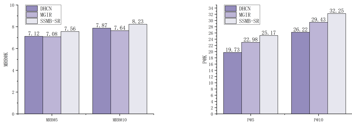
FIGURE 4. Optimized performance comparison for small k values on Nowplaying.
