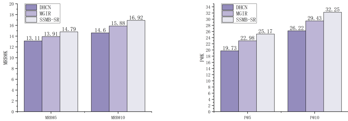
FIGURE 3. Optimized performance comparison for small k values on Tmall.
