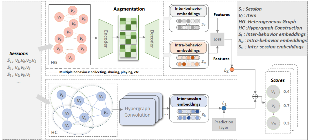
FIGURE 2. The proposed model is structured into two primary components: an upper segment dedicated to the heterogeneous enhancement module and a lower segment comprising the hypergraph module. The heterogeneous enhancement module employs advanced techniques to encapsulate behavioral data, utilizing self-supervised learning to explore the complex interplay of dependencies within and across behaviors. This process integrates diverse behavioral insights, yielding a refined and comprehensive representation of nodes. Additionally, the model incorporates a hypergraph structure, where hypergraph convolutions are applied to capture and exploit the intricate, high-order relationships among items. In the final stage, the model funnels these insights into a specialized prediction module, which produces probabilistic predictions for candidate items.
